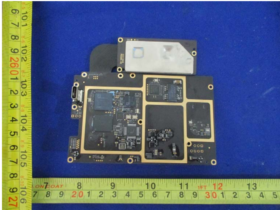
EUT – RF Board Bottom View
