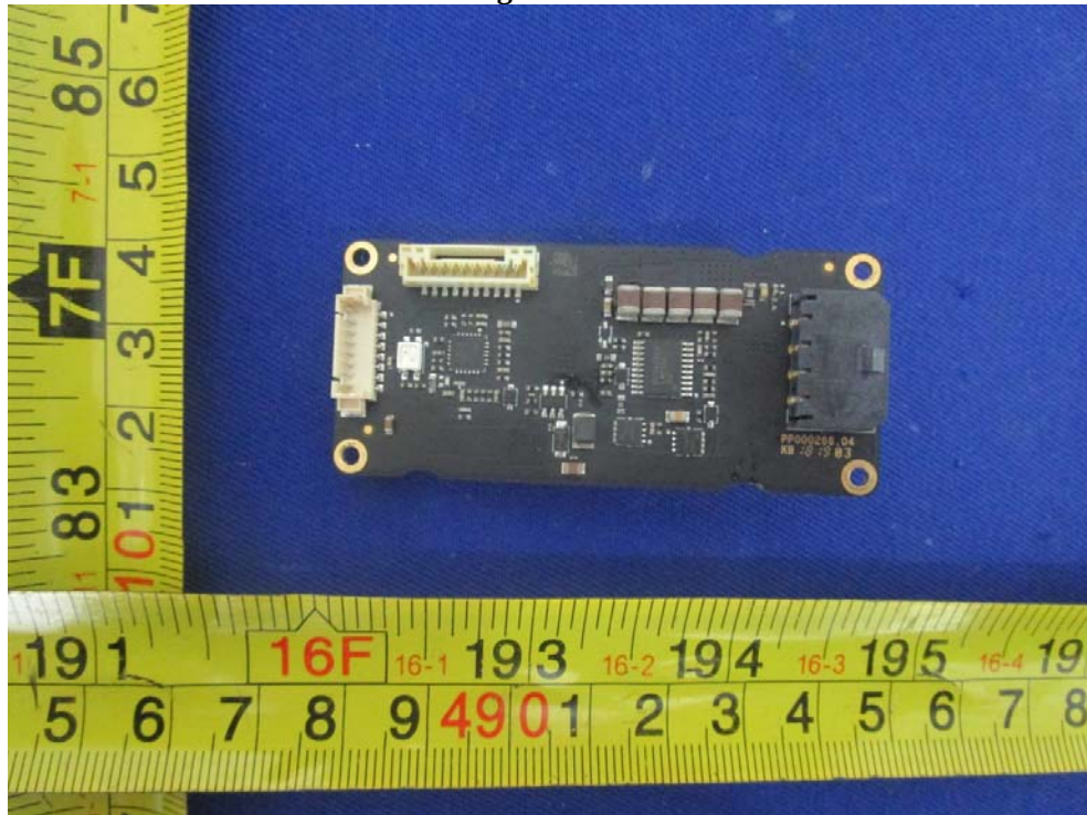
EUT – Power Management Board Bottom View
