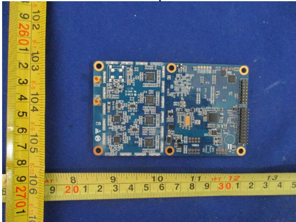
EUT – RTK Module Top Unshielded View
