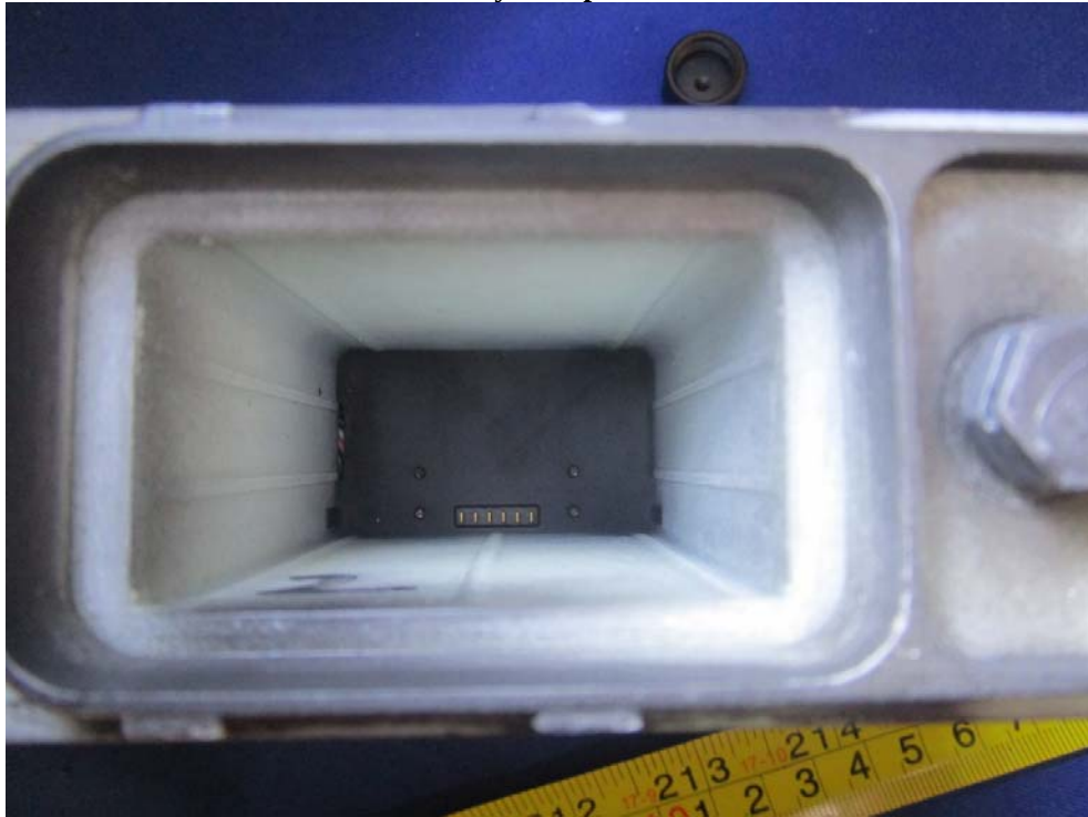
EUT – Battery Compartment View
