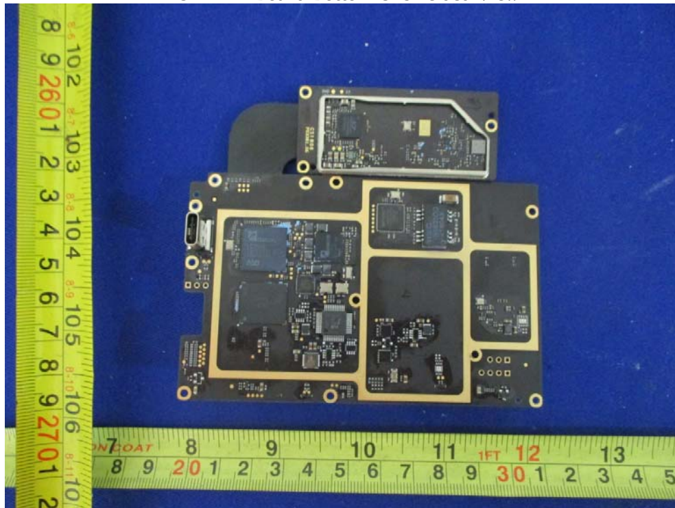
EUT – RF Board Bottom Unshielded View
