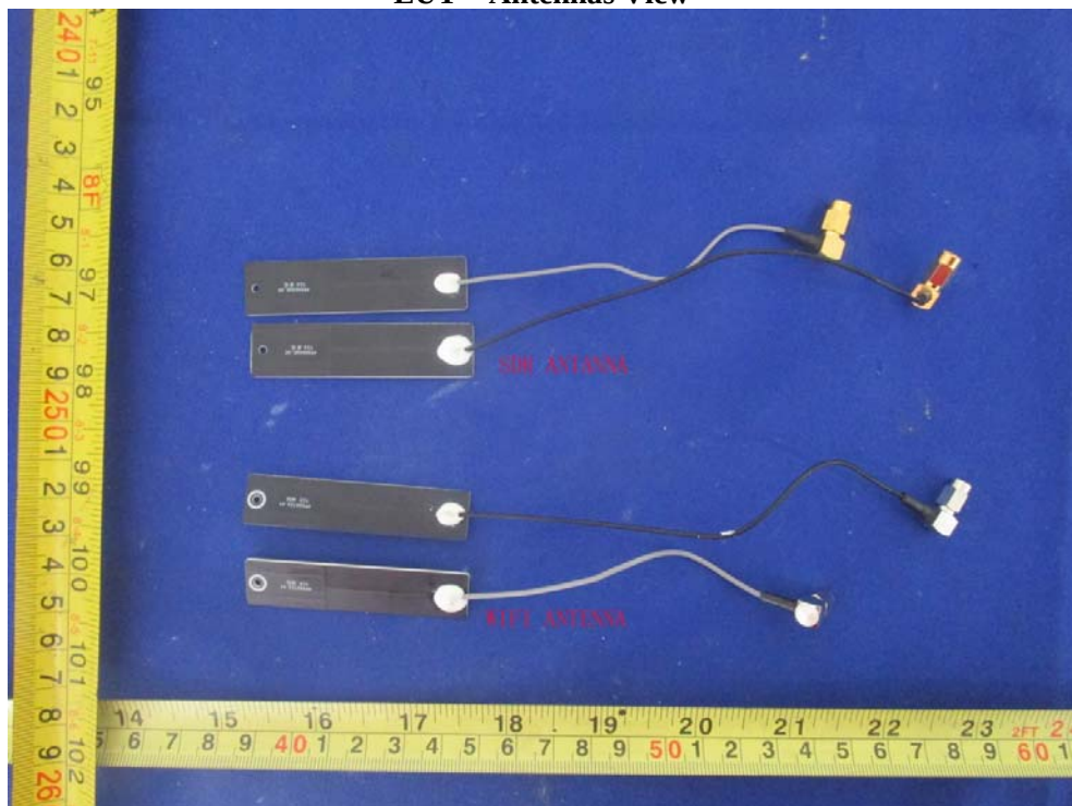
EUT – Antennas View
