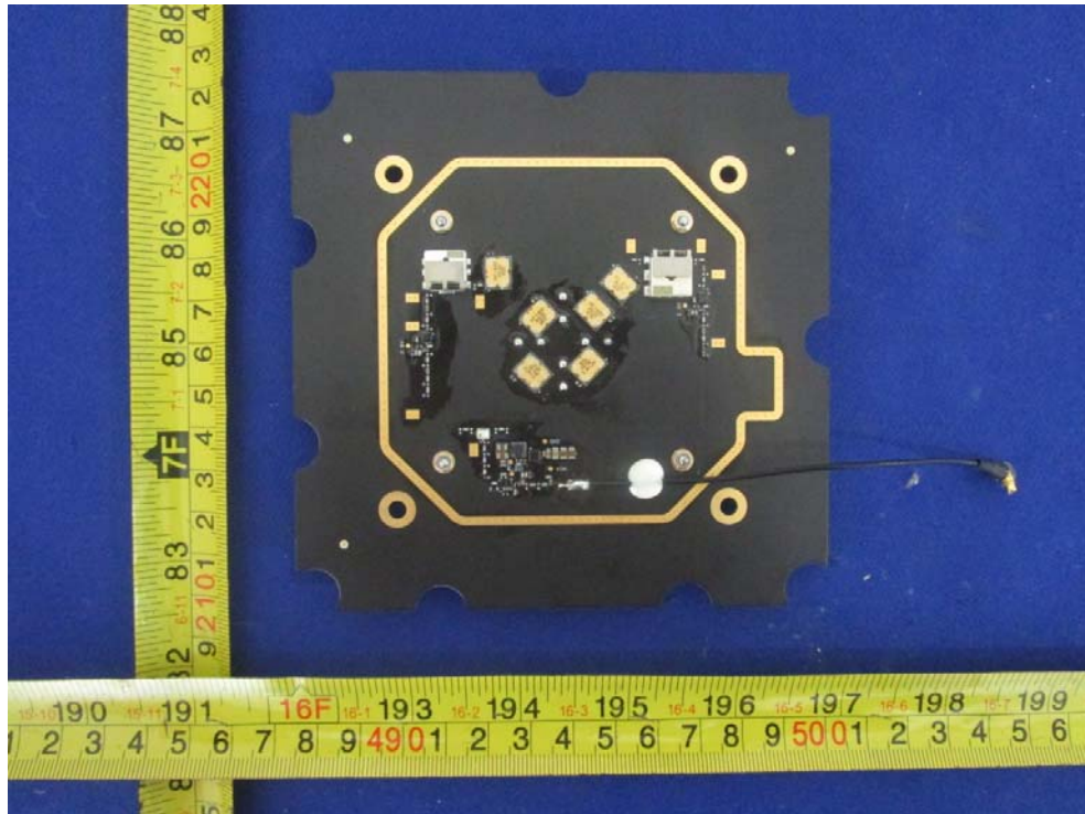
EUT – RTK Antenna Bottom View
