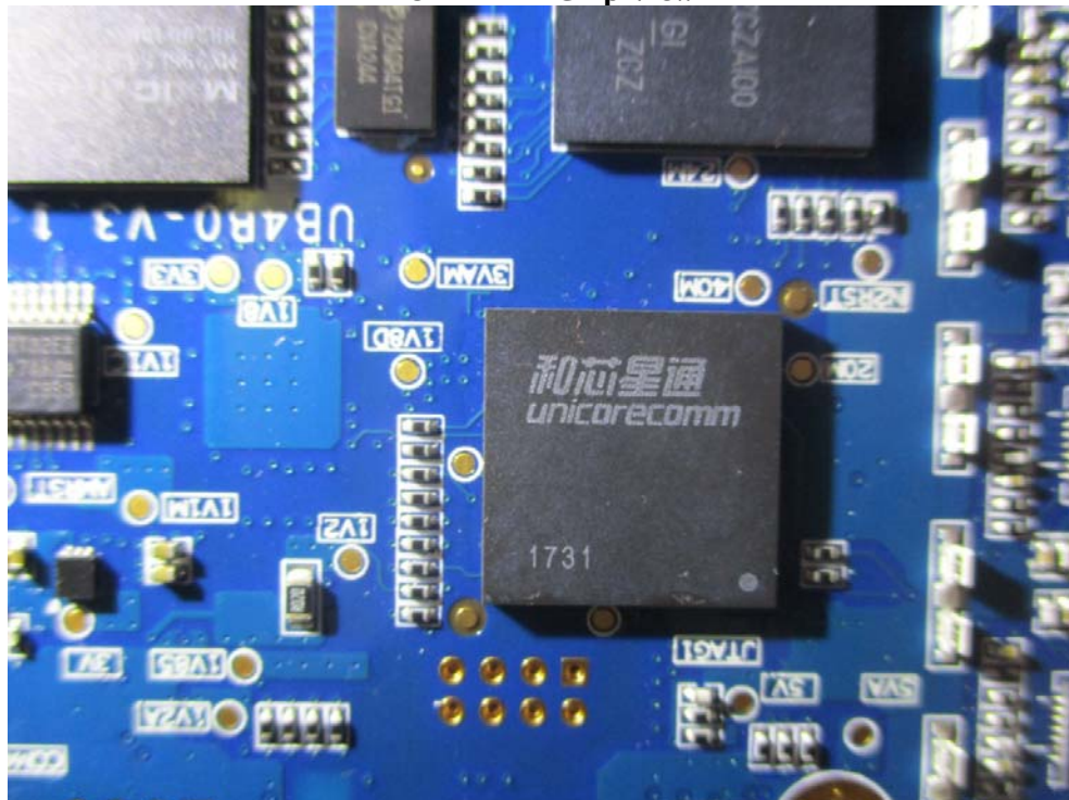
EUT – RTK Chip View
