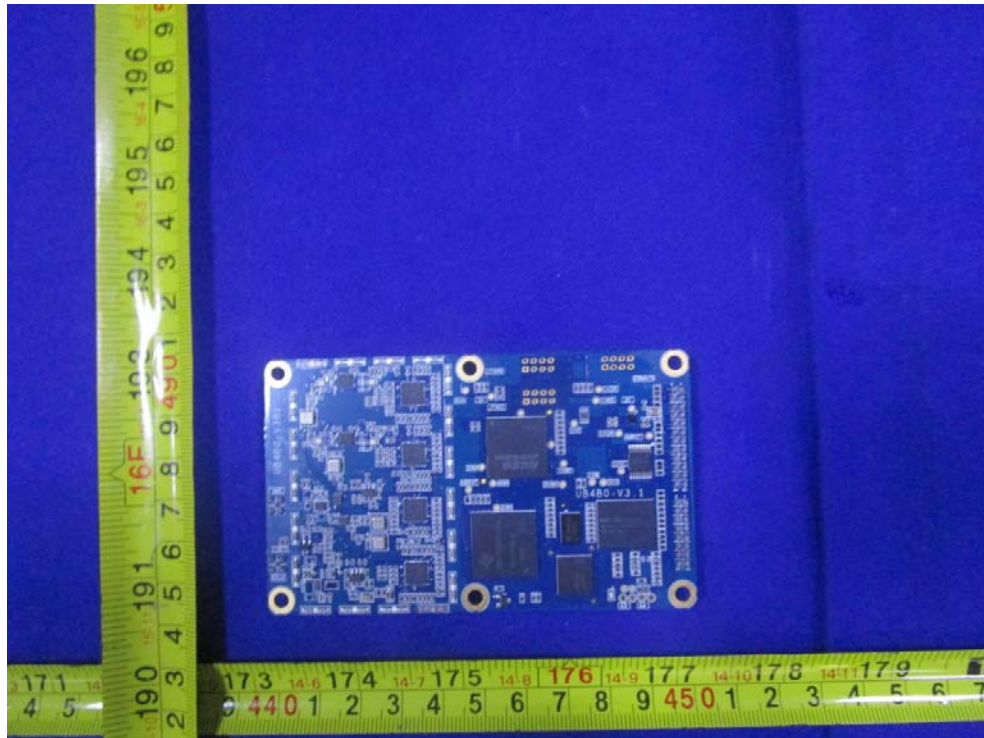
EUT – RTK Module Bottom Unshielded View
