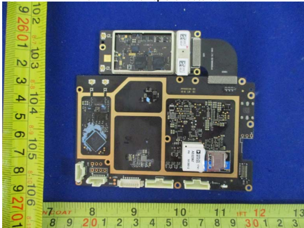
EUT – RF Board Top Unshielded View
