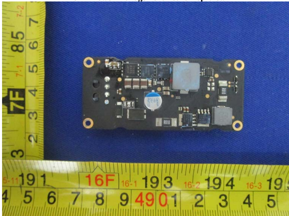
EUT – Power Management Board Top View
