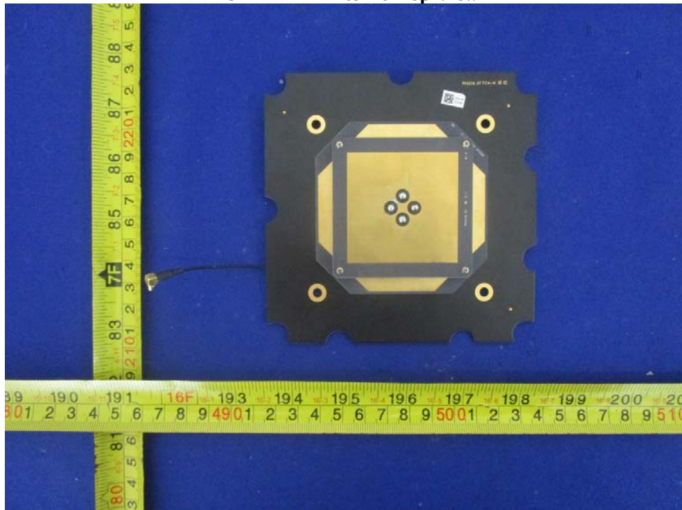
EUT – RTK Antenna Top View
