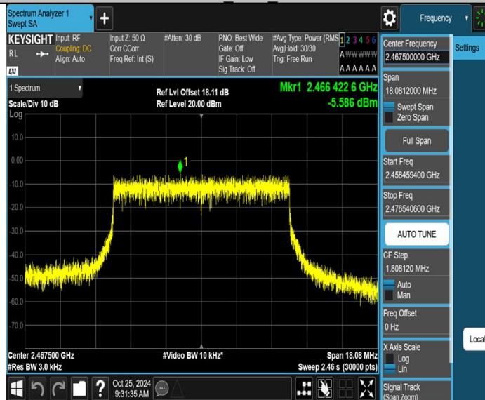
10MHz Ant2 2467.5
