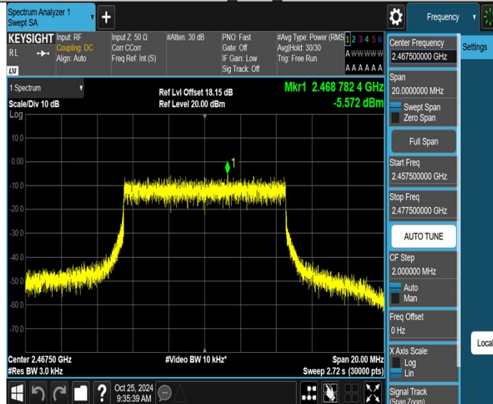
10MHz Ant2 2467.5
