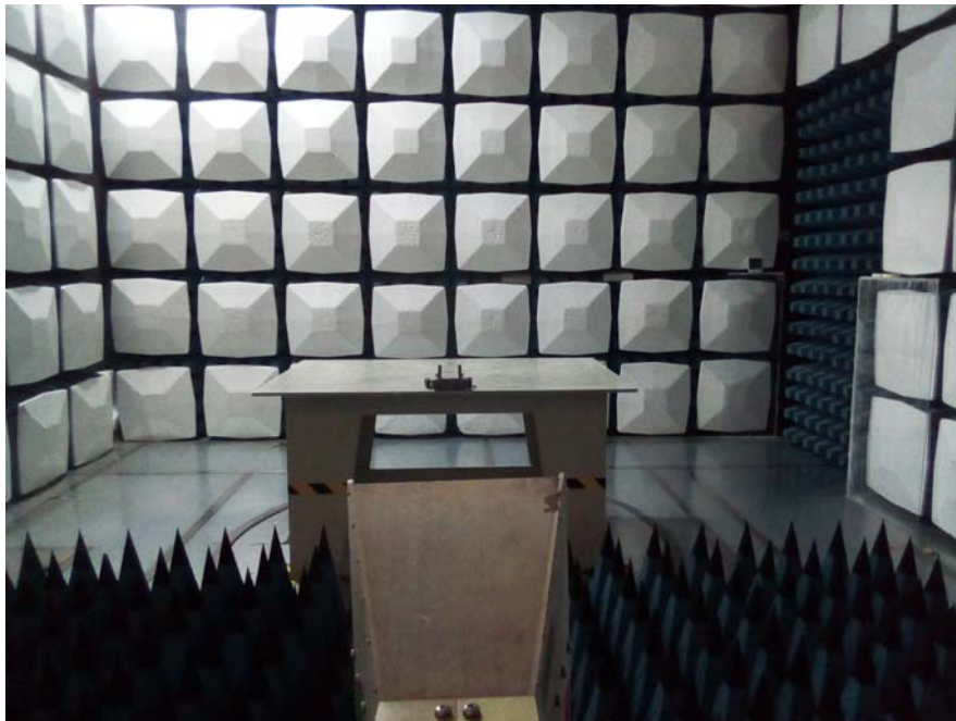
RE Above 1G Rear View(Operating with Micro USB)
