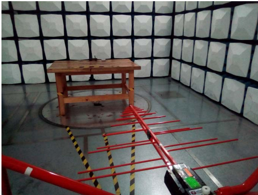
RE Below 1G Rear View(Operating with USB-A)
