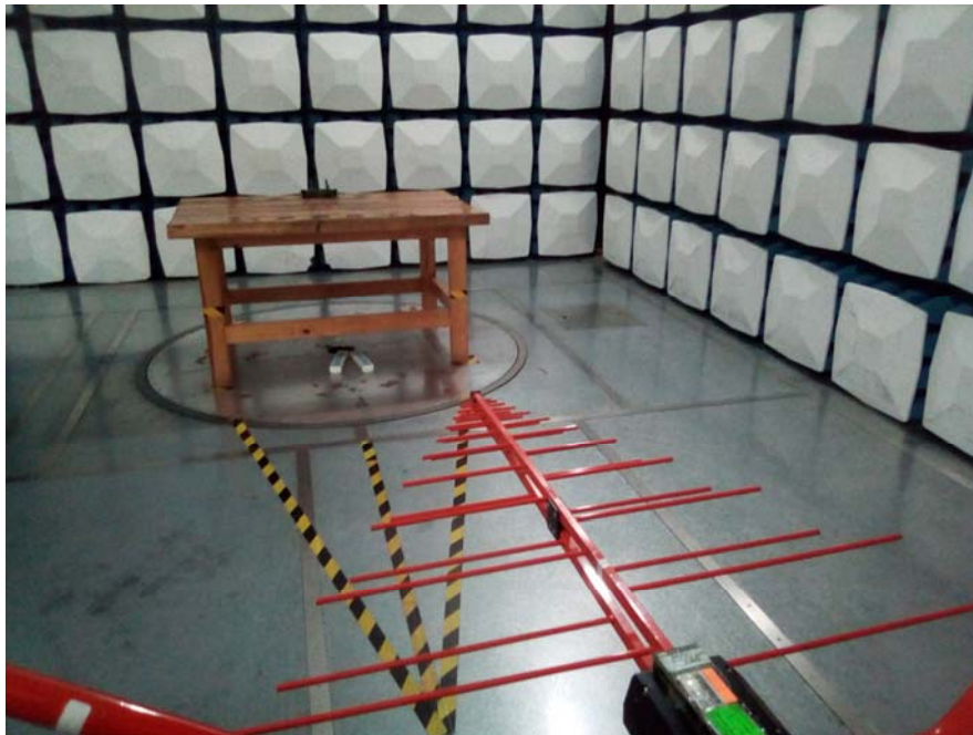
RE Below 1G Front View(Operating with Micro USB)
