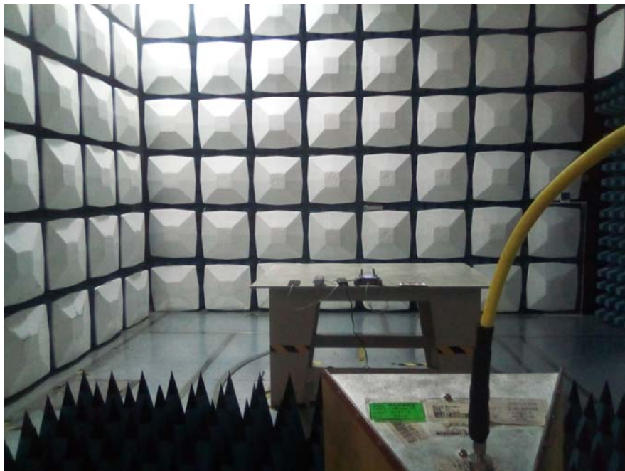
RE Above 1G Rear View(charging)
