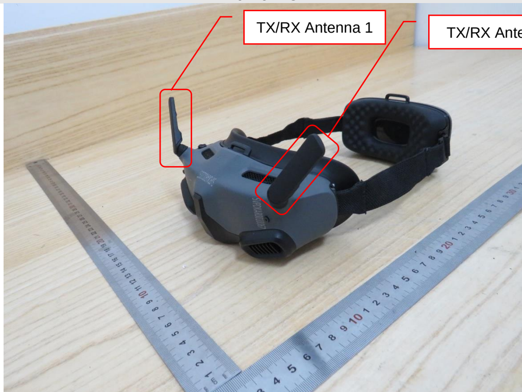
View of EUT
