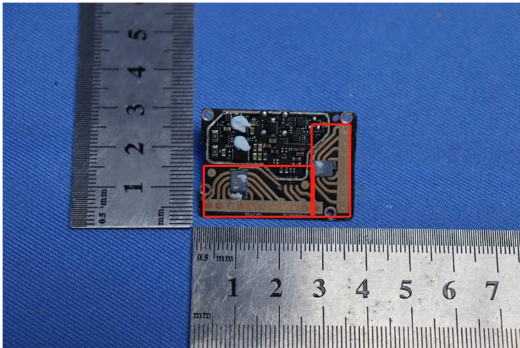
Antenna Location
