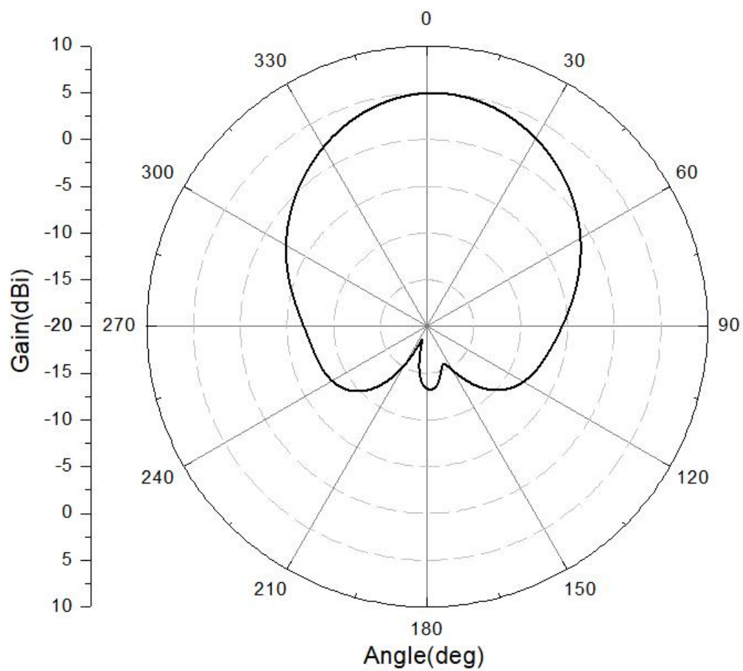
b) H Plane
