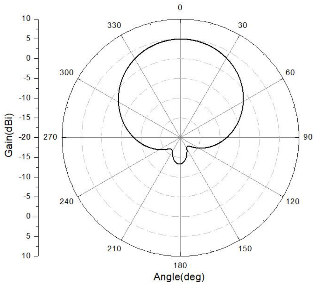
a) E Plane
