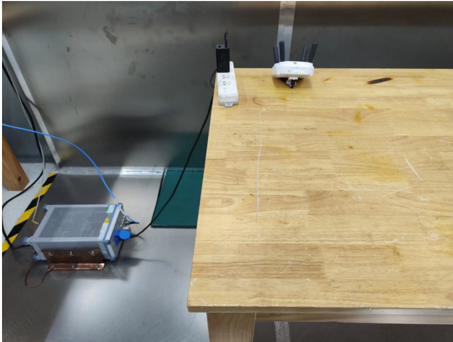
Photograph 3: Set-up photo for AC Conducted Emissions
