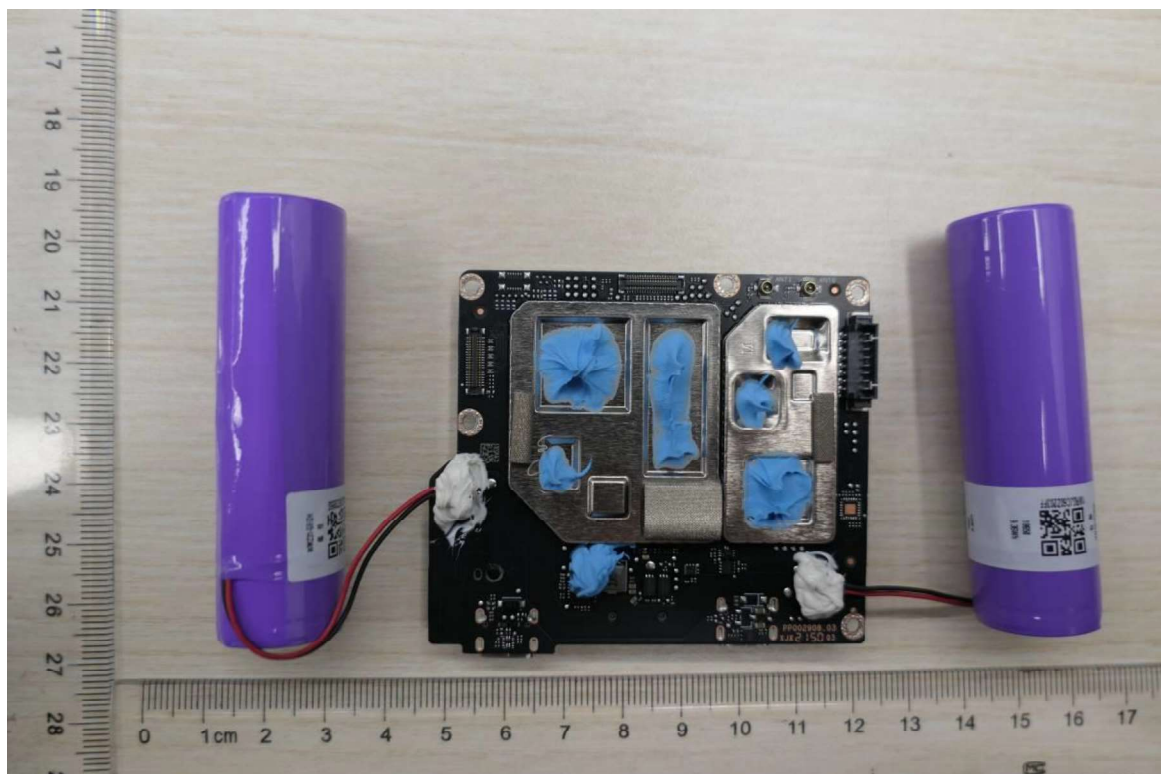
Figure 8 PCB view 1
