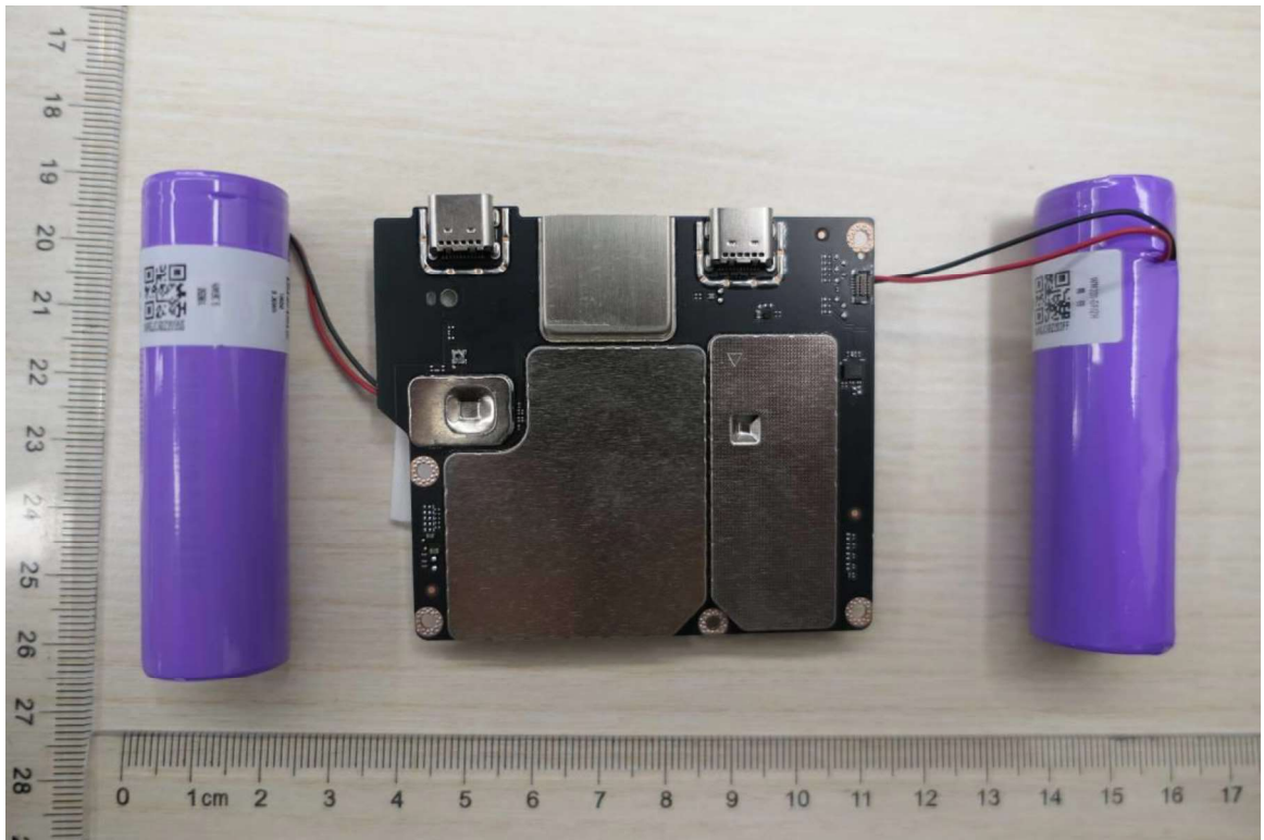
Figure 9 PCB view 2
