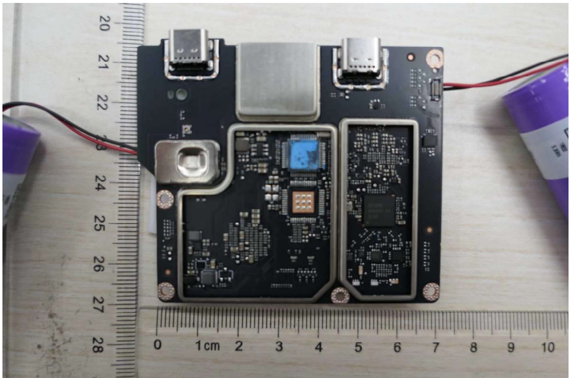
Figure 10 PCB view 3
