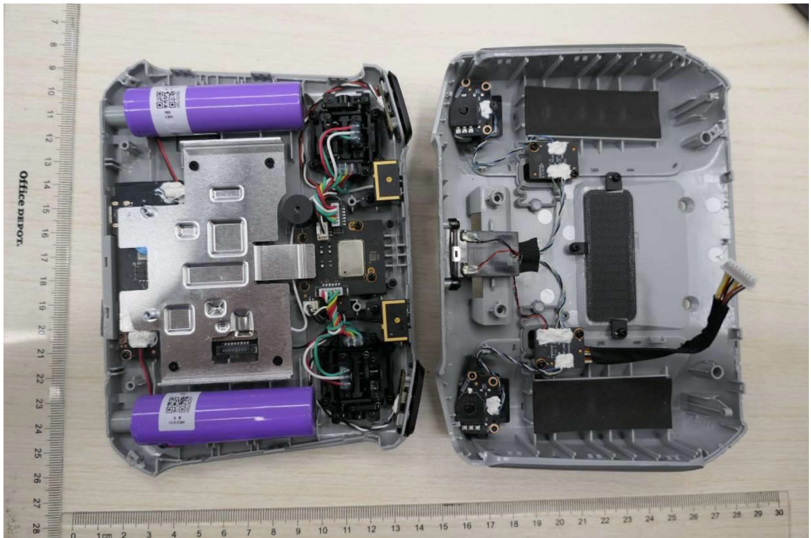
Figure 5 Internal view 1
