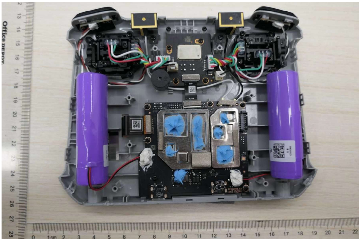
Figure 6 Internal view 2
