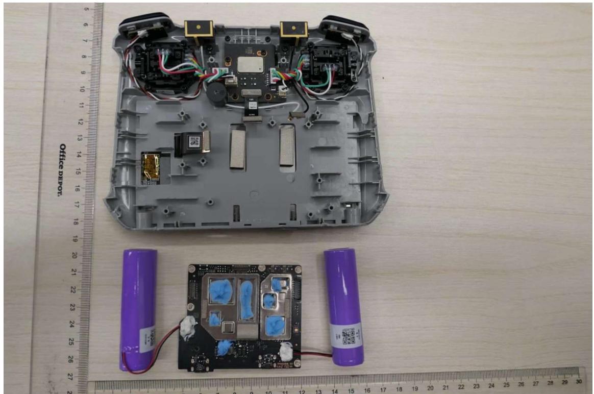
Figure 7 Internal view 3
