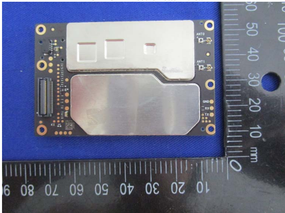
EUT – SDR Module Bottom View
