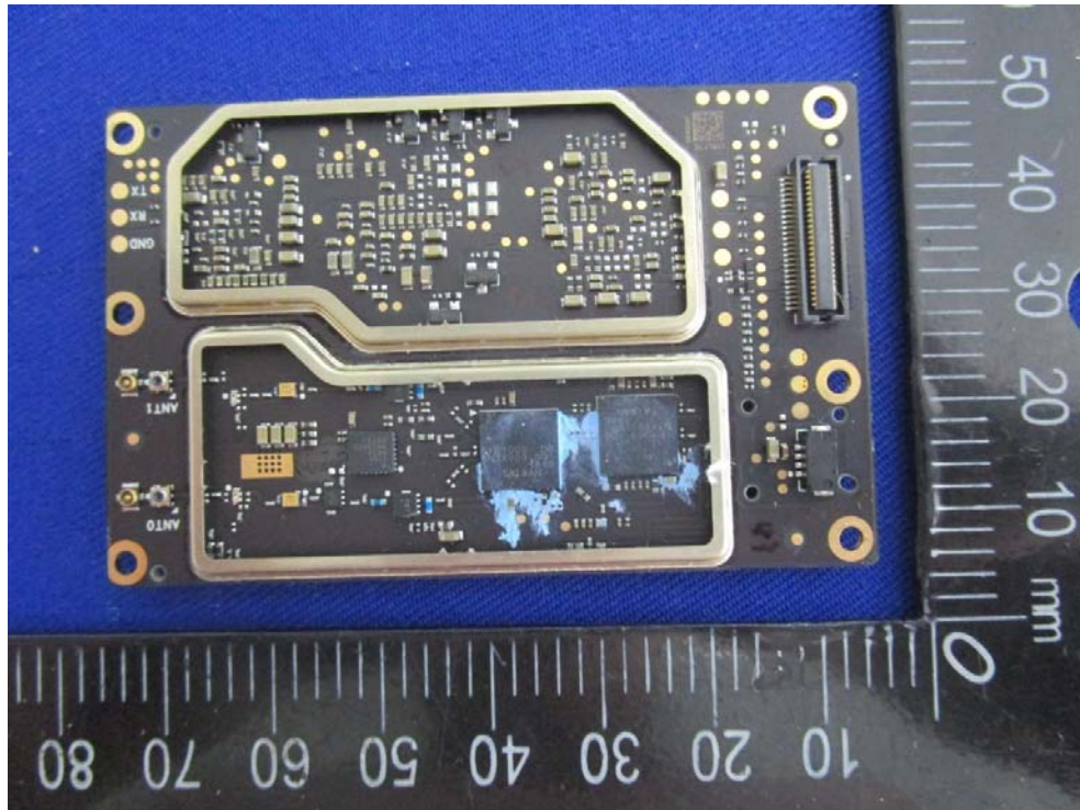
EUT – SDR Module Bottom Unshielded View
