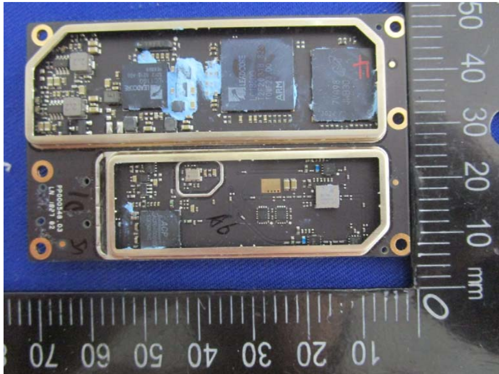
EUT – SDR Module Unshiled View
