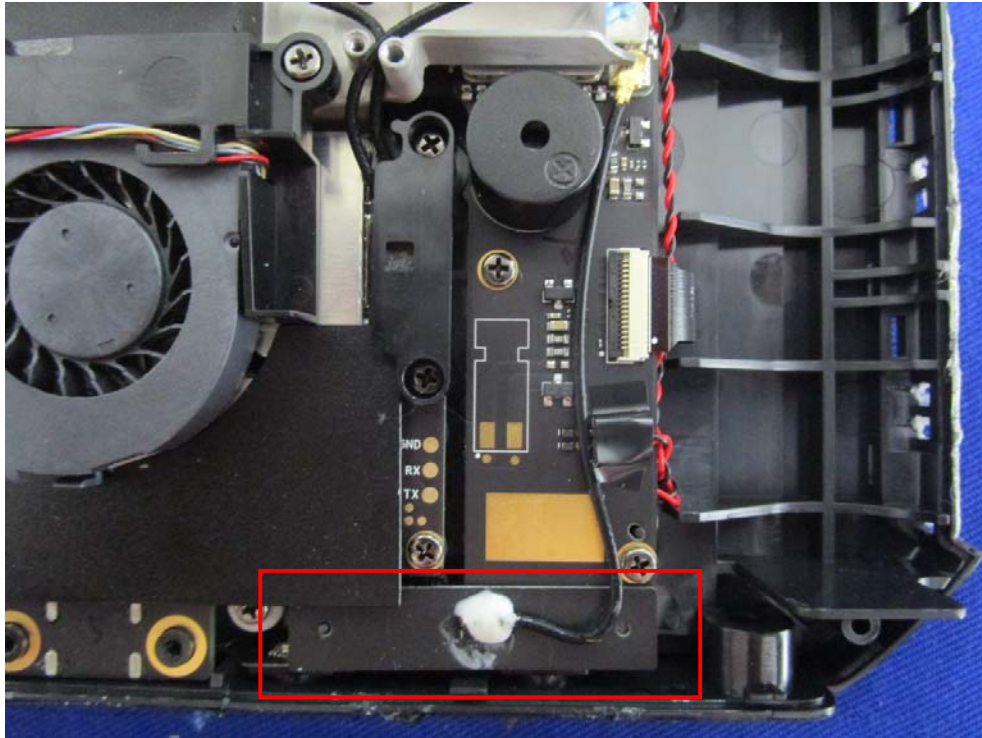
EUT – Wifi/Bluetooth Chain 1 Antenna View
