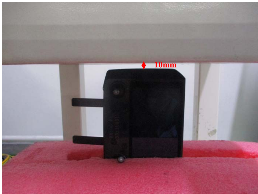
Test Position_Right (10mm)
