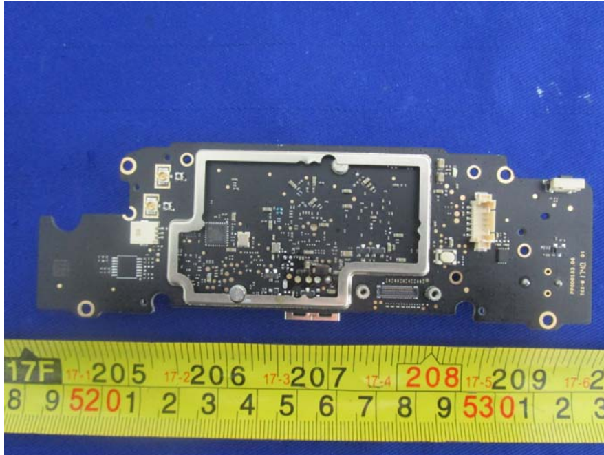
EUT – PCB 2 Top Uncover View
