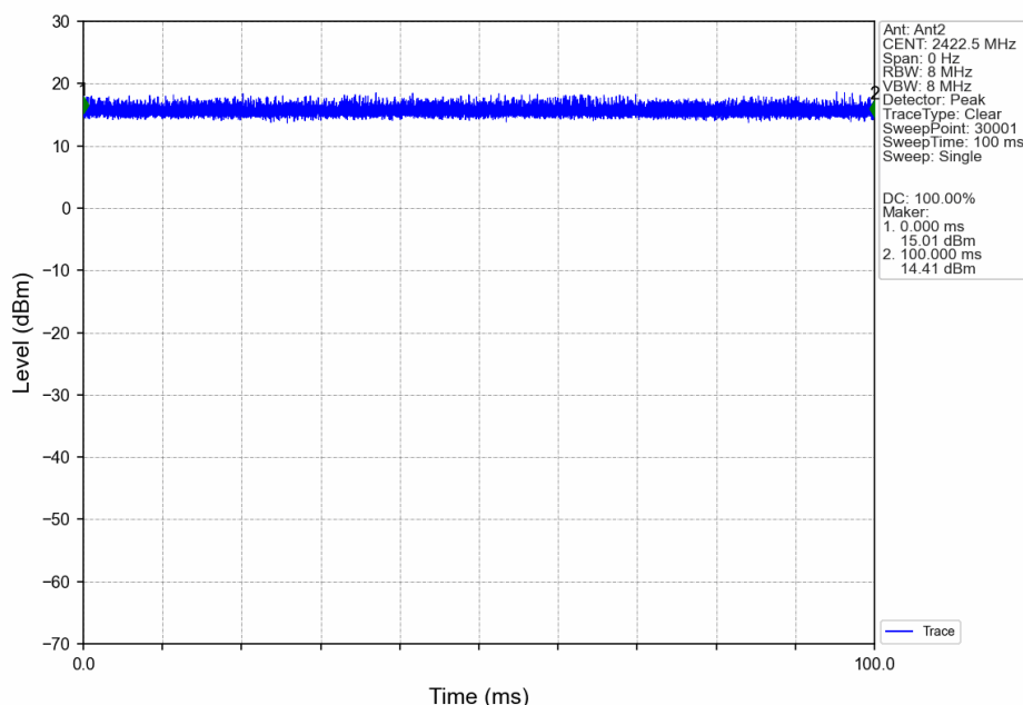
40M_LCH_2422.5MHz_Ant2_NTNV
