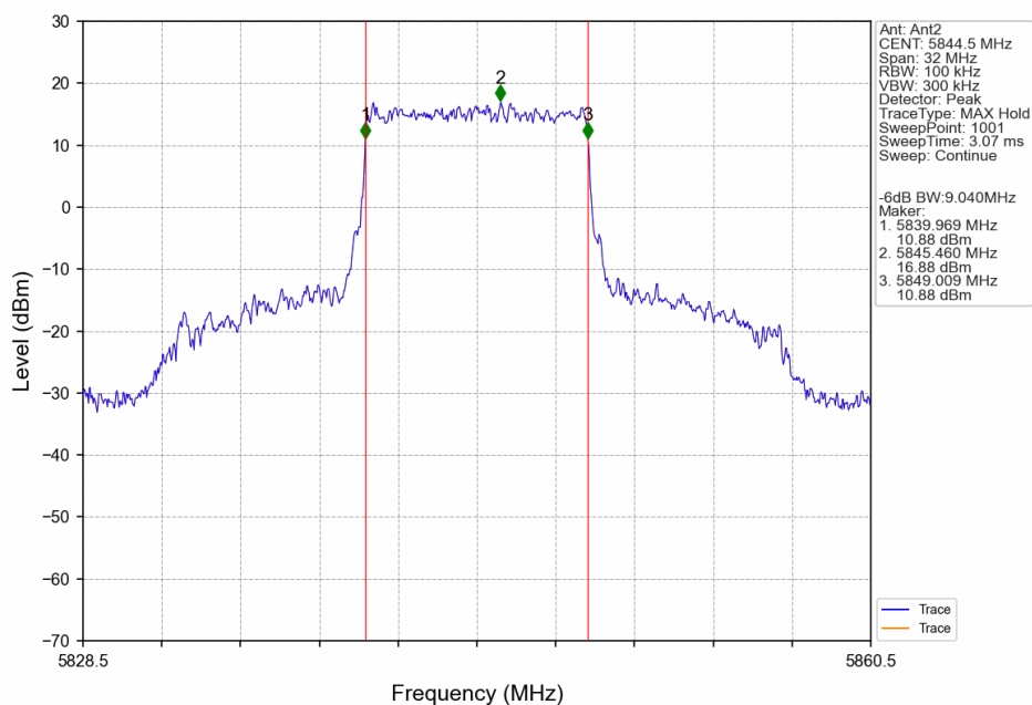
10M_HCH_5844.5MHz_Ant2_NTNV
