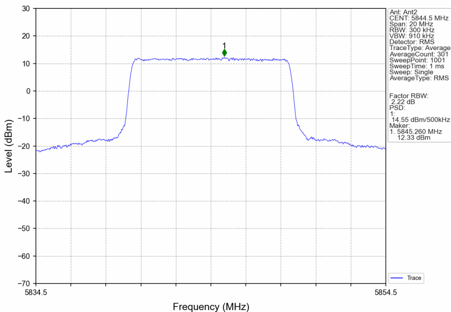
10M_HCH_5844.5MHz_Ant2_NTNV
