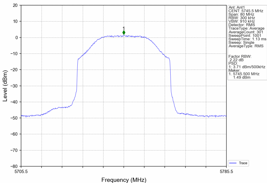
40M_LCH_5745.5MHz_MIMO_NTNV
