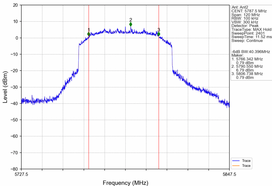
60M_MCH_5787.5MHz_Ant2_NTNV
