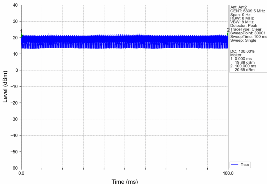
80M_HCH_5809.5MHz_Ant2_NTNV
