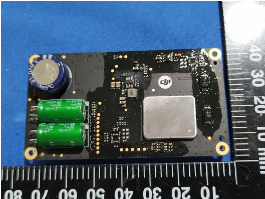
GPS Board
