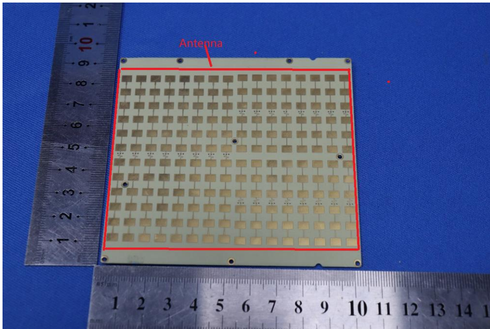
Antenna for Omnidirectional radar
