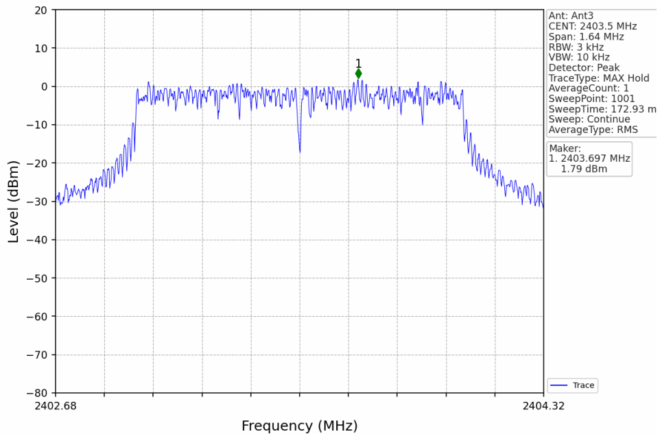
1.4M_LCH_2403.5MHz_Ant3_NTNV
