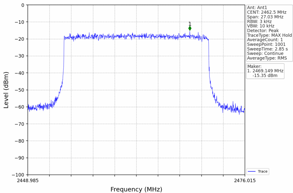
20M_HCH_2462.5MHz_Ant1_NTNV
