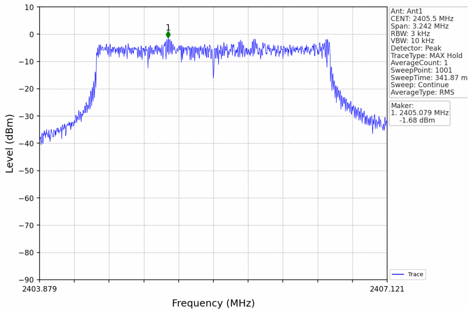
3M_LCH_2405.5MHz_Ant1_NTNV
