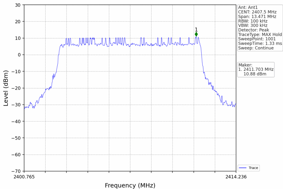
10M_LCH_2407.5MHz_Ant1_NTNV
