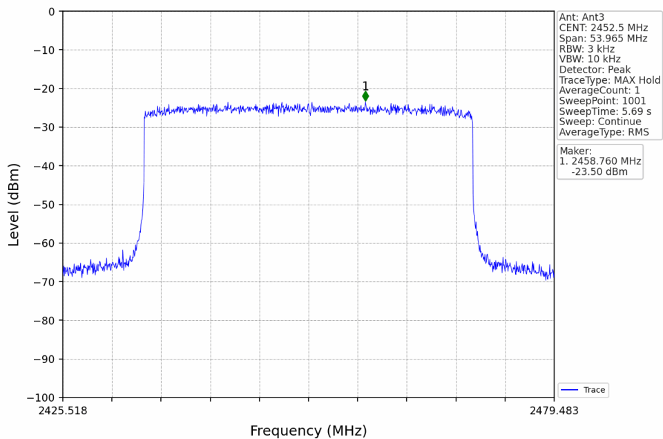
40M_HCH_2452.5MHz_Ant3_NTNV
