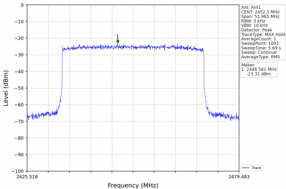
40M_HCH_2452.5MHz_Ant1_NTNV
