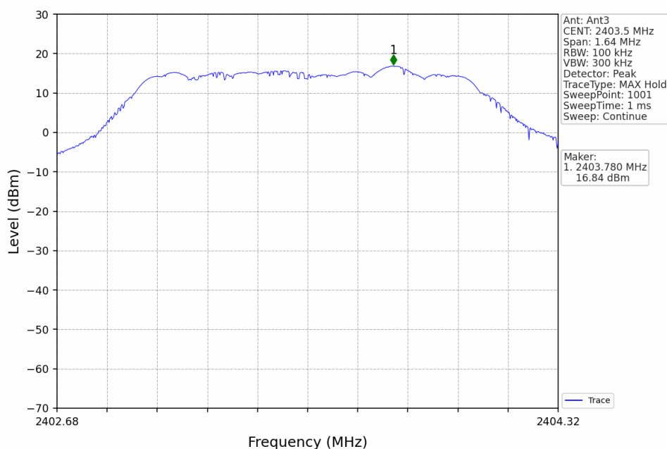
1.4M_LCH_2403.5MHz_Ant3_NTNV
