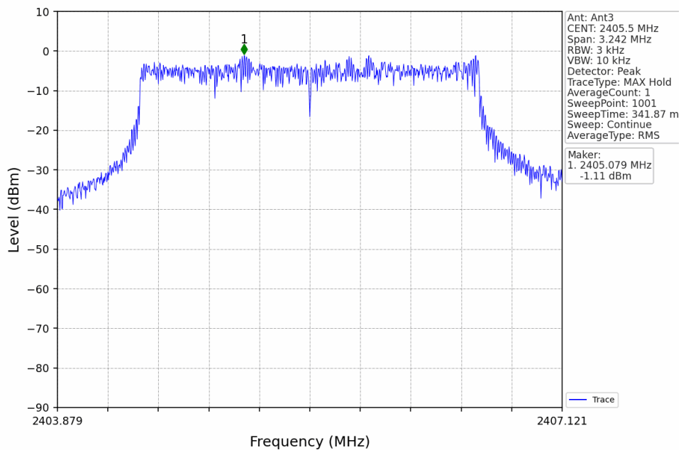
3M_LCH_2405.5MHz_Ant3_NTNV
