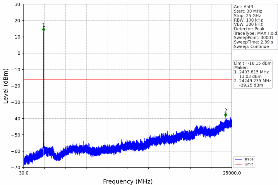
1.4M_LCH_2403.5MHz_Ant3_NTNV
