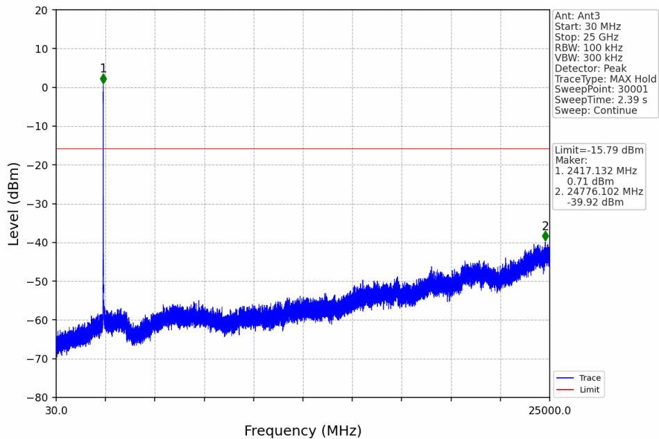
20M_LCH_2412.5MHz_Ant3_NTNV
