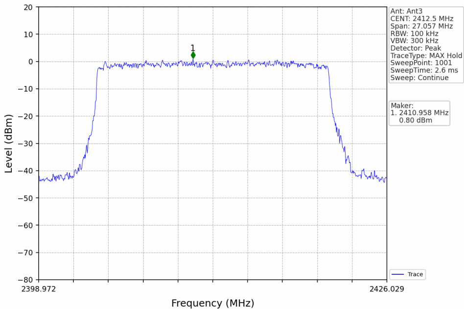
20M_LCH_2412.5MHz_Ant3_NTNV
