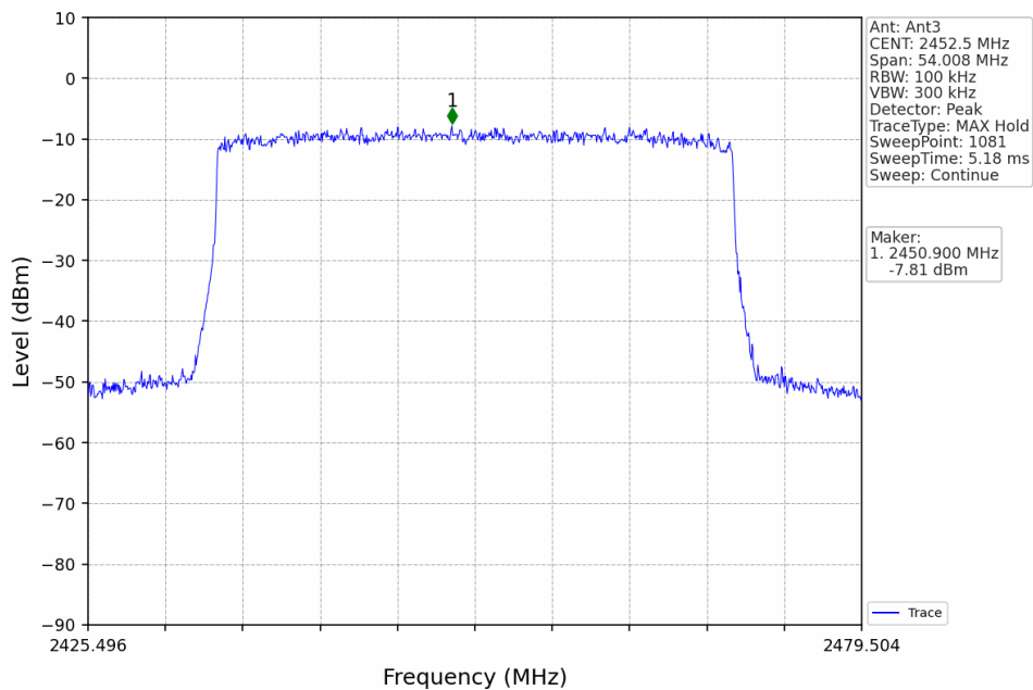
40M_HCH_2452.5MHz_Ant3_NTNV
