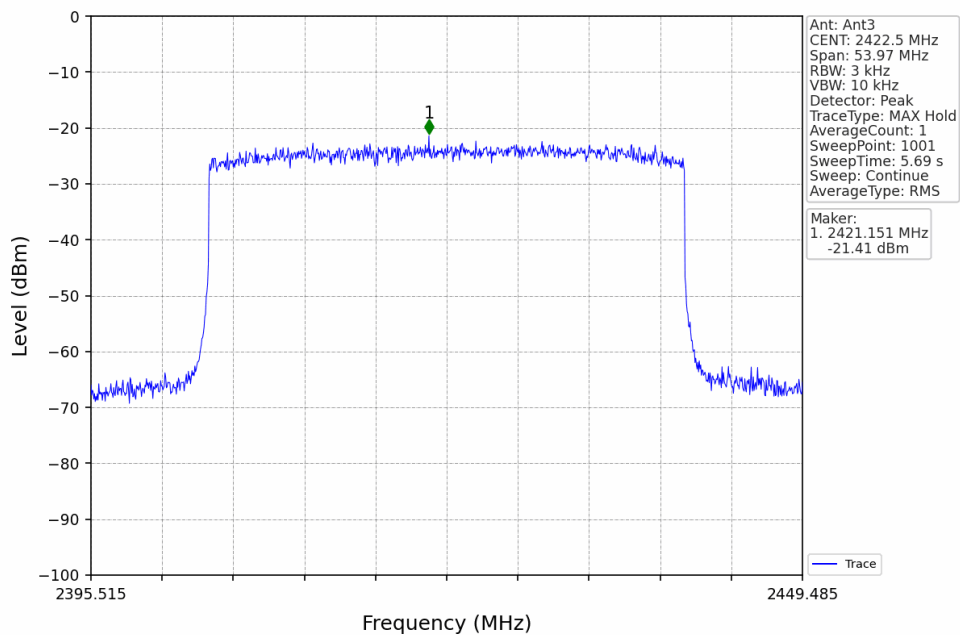
40M_LCH_2422.5MHz_Ant3_NTNV
