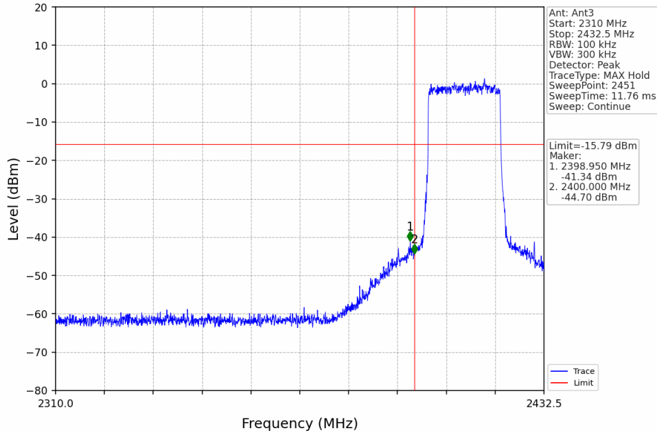
20M_LCH_2412.5MHz_Ant3_NTNV
