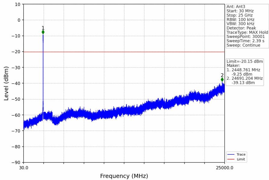
40M_HCH_2452.5MHz_Ant3_NTNV
