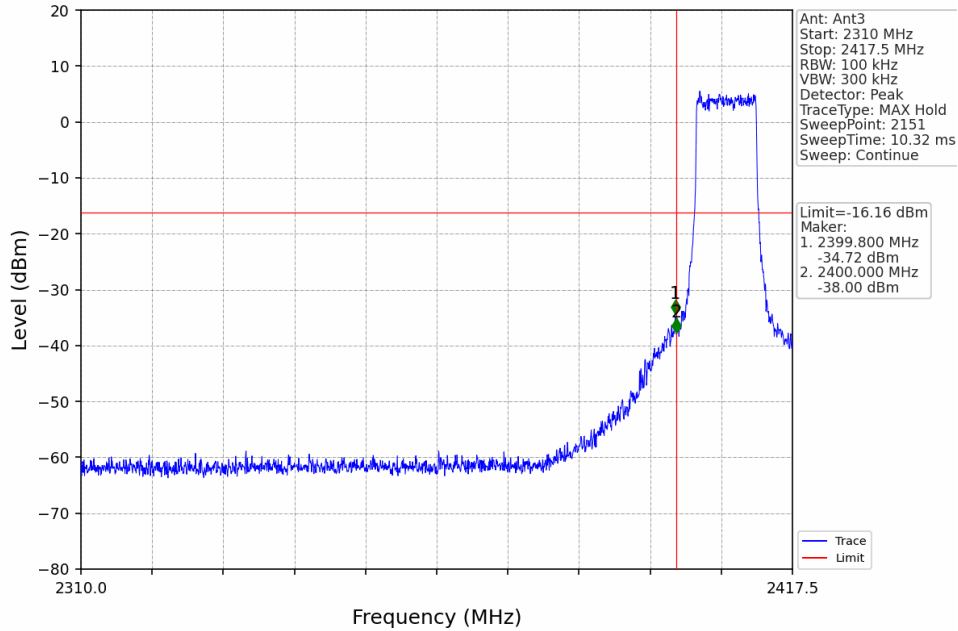
10M_LCH_2407.5MHz_Ant3_NTNV
