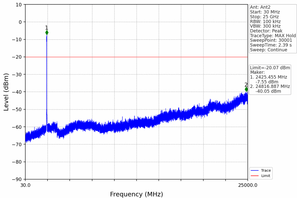
40M_LCH_2422.5MHz_Ant2_NTNV
