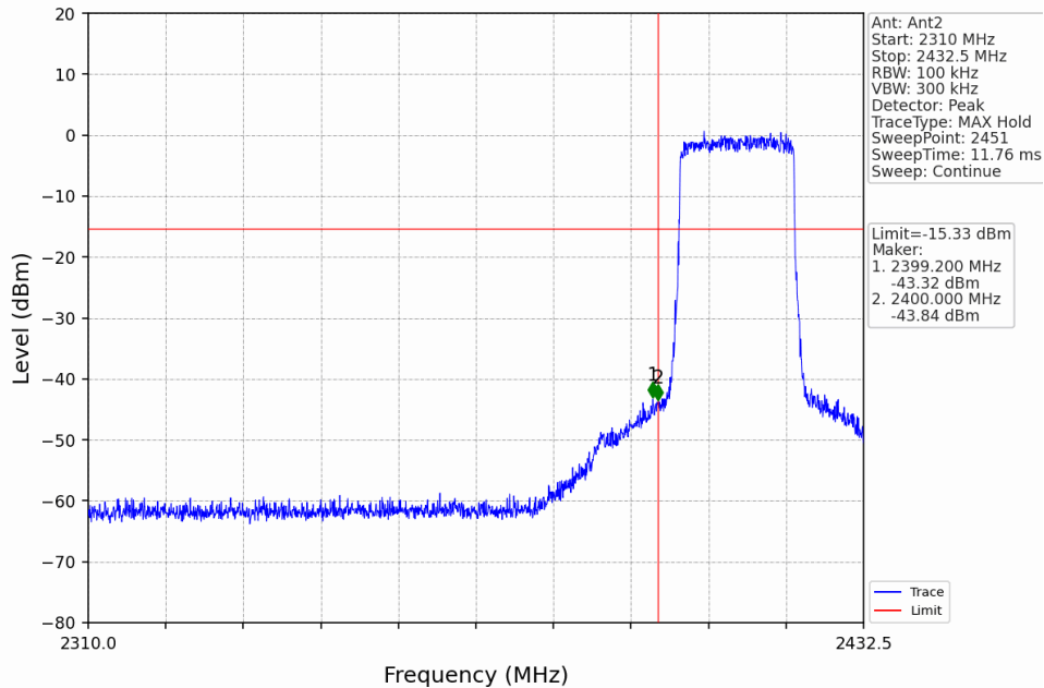
20M_LCH_2412.5MHz_Ant2_NTNV
