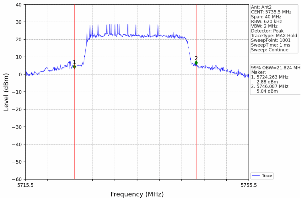
20M_LCH_5735.5MHz_Ant2_NTNV
