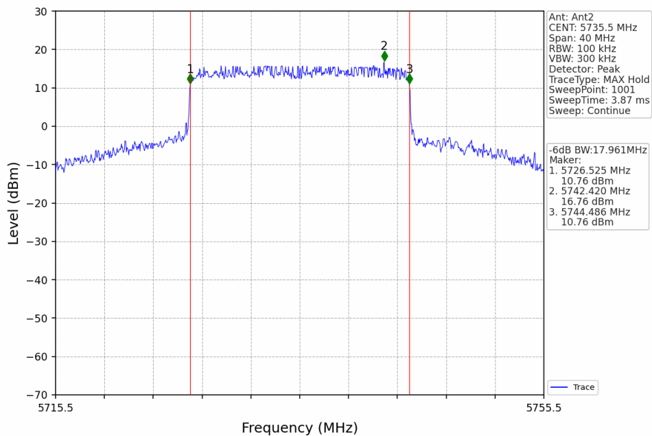
20M_LCH_5735.5MHz_Ant2_NTNV
