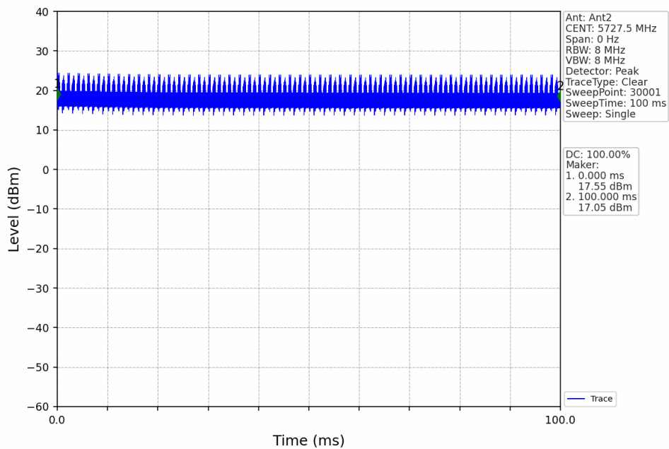
3M_LCH_5727.5MHz_Ant2_NTNV
