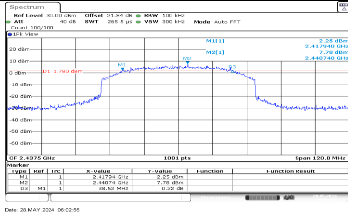
SRD 60M Ant2 2437.5
