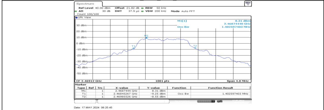
SRD_1.4M_Ant2_2469.12
