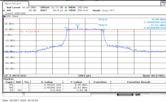
SRD 10M Ant2 2407.5
