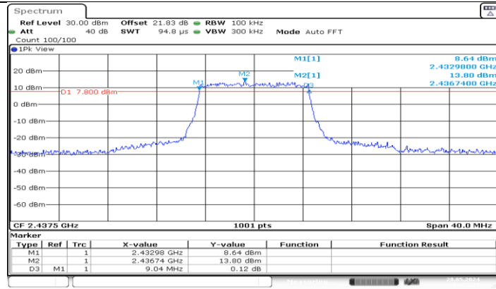
SRD 10M Ant1 2437.5
