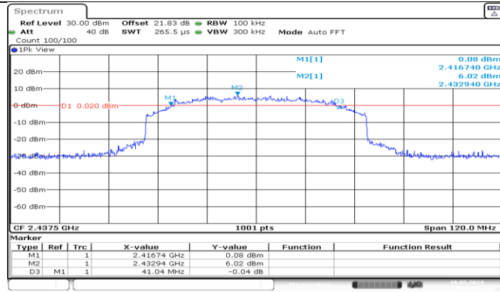
SRD 60M Ant1 2437.5
