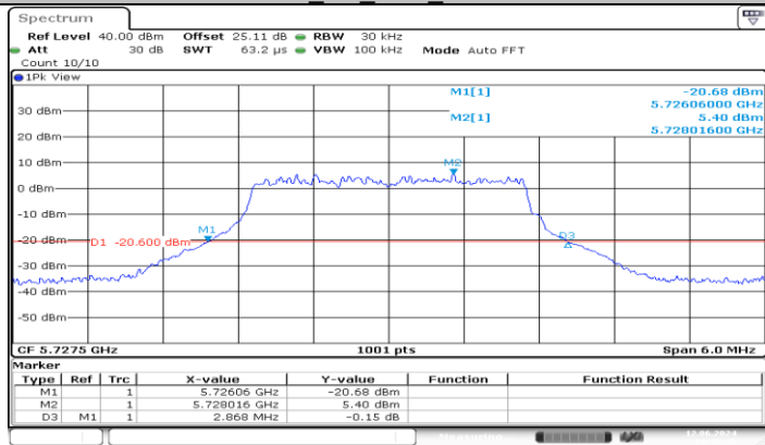
SRD_3M_Ant1_5727.5
