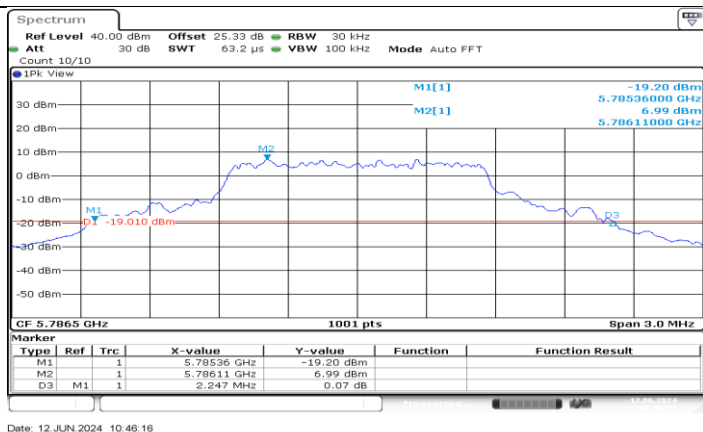
SRD_1.4M_Ant2_5786.5
