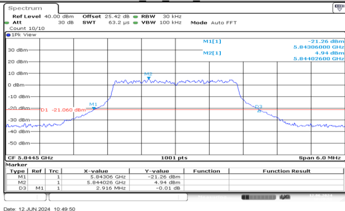
SRD_3M_Ant1_5844.5
