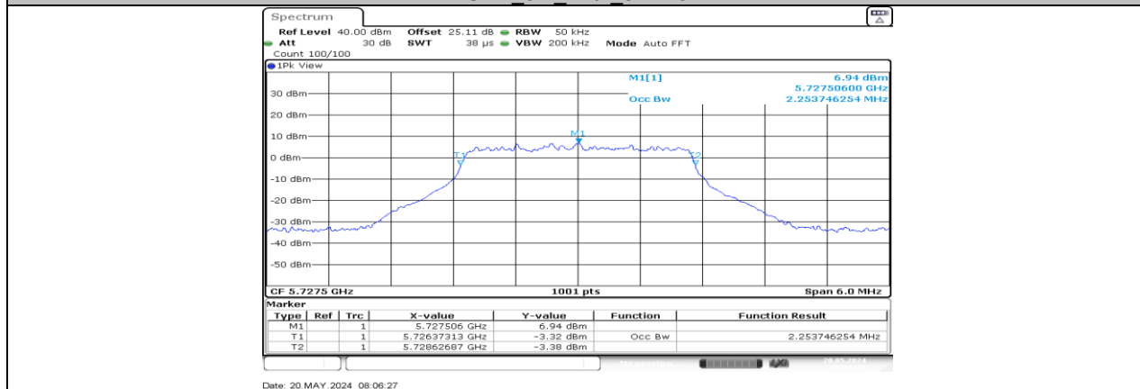
SRD_3M_Ant2_5727.5
