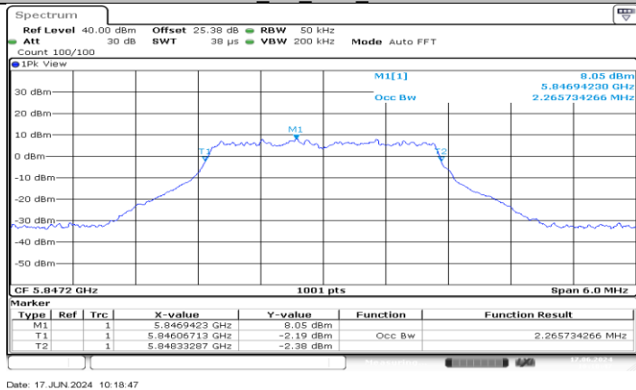
SRD_3M_Ant2_5847.2
