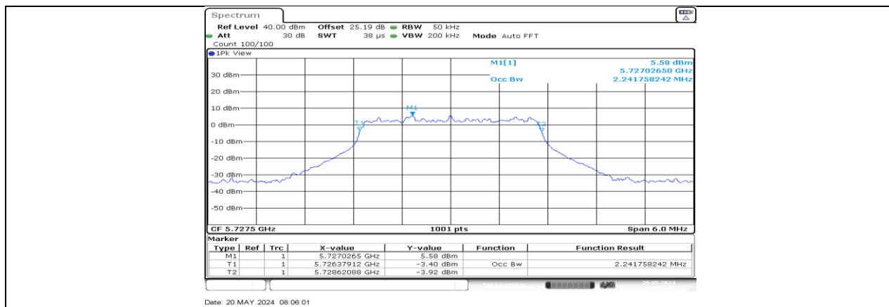
SRD_3M_Ant1_5727.5
