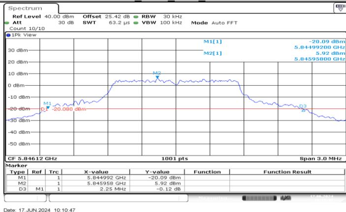
SRD_1.4M_Ant1_5846.12
