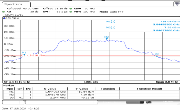
SRD_1.4M_Ant2_5846.12
