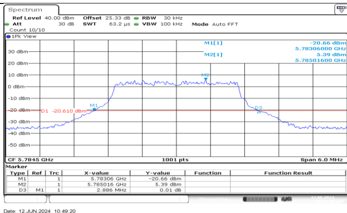
SRD_3M_Ant2_5784.5
