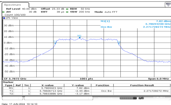
SRD_3M_Ant2_5787.2
