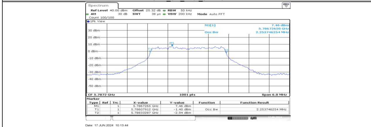
SRD_3M_Ant1_5787.2
