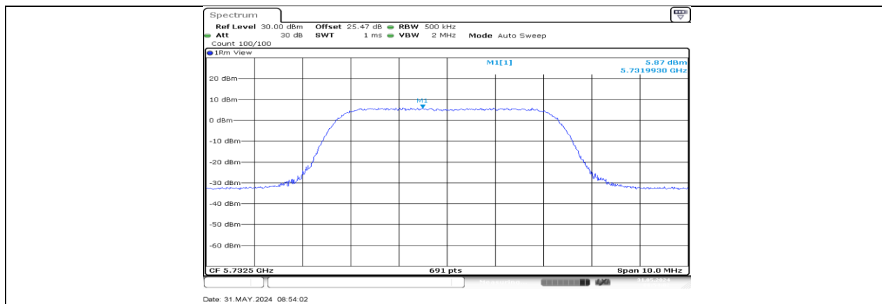
SRD_5M_Ant1_5732.5
