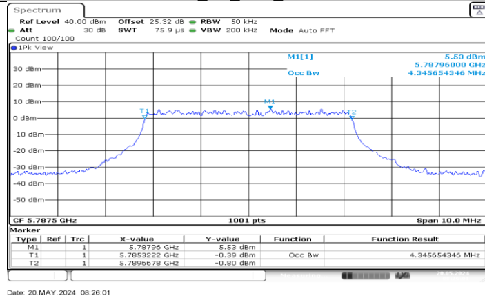
SRD_5M_Ant1_5787.5
