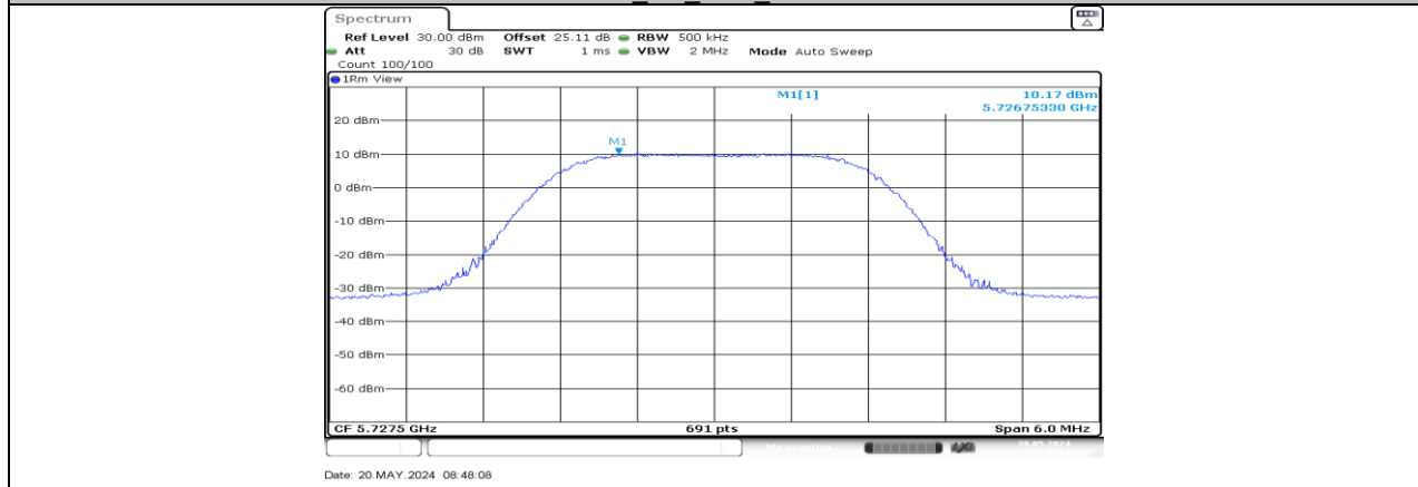
SRD_3M_Ant2_5727.5
