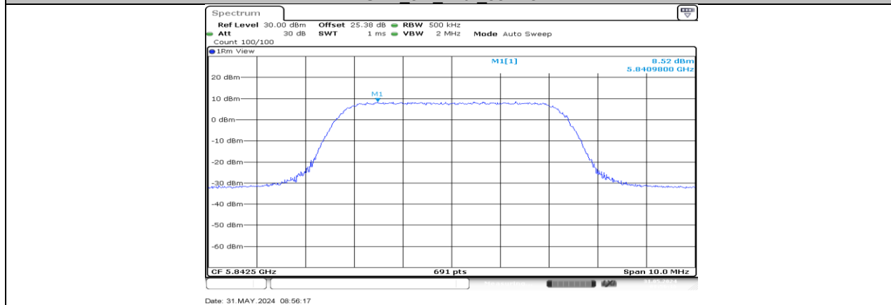
SRD_5M_Ant2_5842.5
