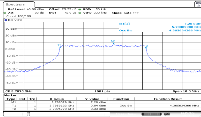
SRD_5M_Ant2_5787.5
