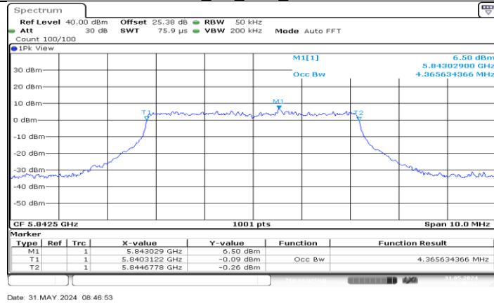
SRD_5M_Ant2_5842.5
