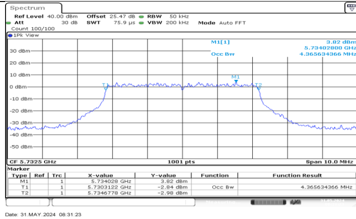
SRD_5M_Ant1_5732.5
