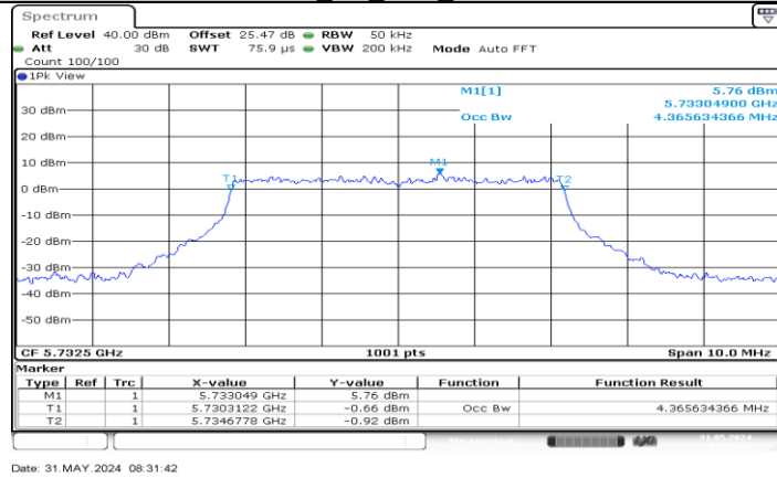
SRD_5M_Ant2_5732.5
