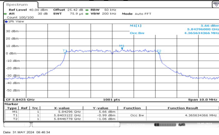
SRD_5M_Ant1_5842.5
