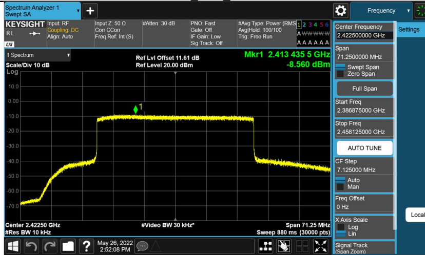
40M_Ant1_2422.5
