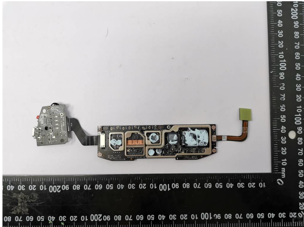
Fig.4. Internal view 4
