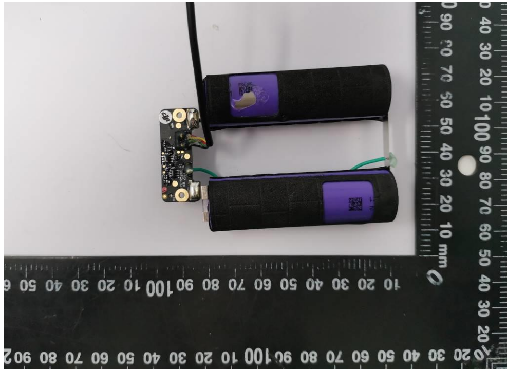
Fig.6. PCB view 1
