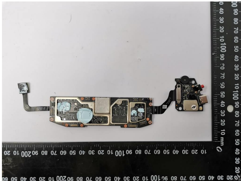
Fig.5. Internal view 5
