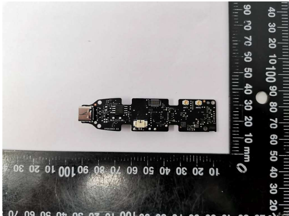
Fig.9. PCB view 1
