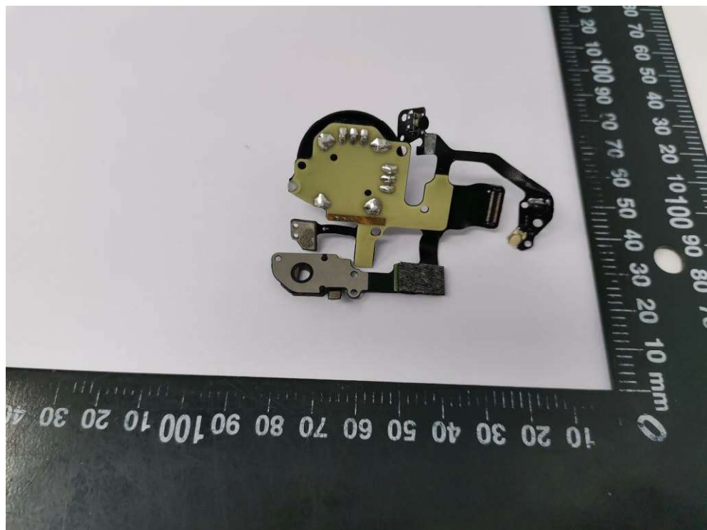
Fig.12. PCB view 4
