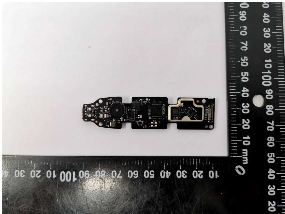
Fig.10. PCB view 2
