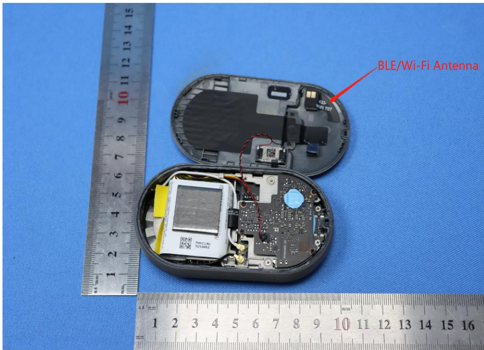
Antenna Location
