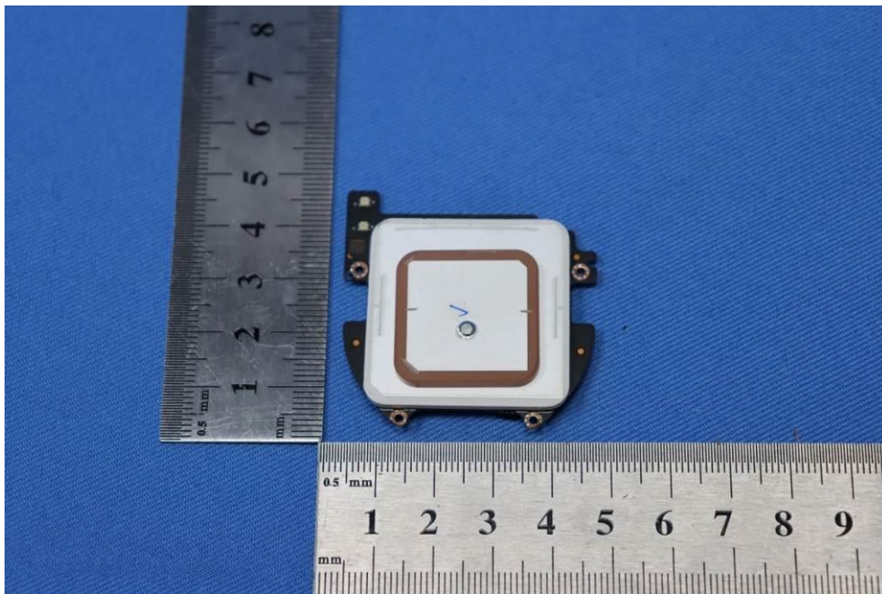
Antenna Location
