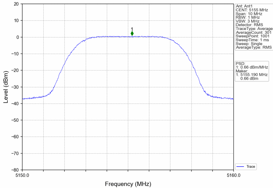
5M_LCH_5155MHz_Ant1_NTNV
