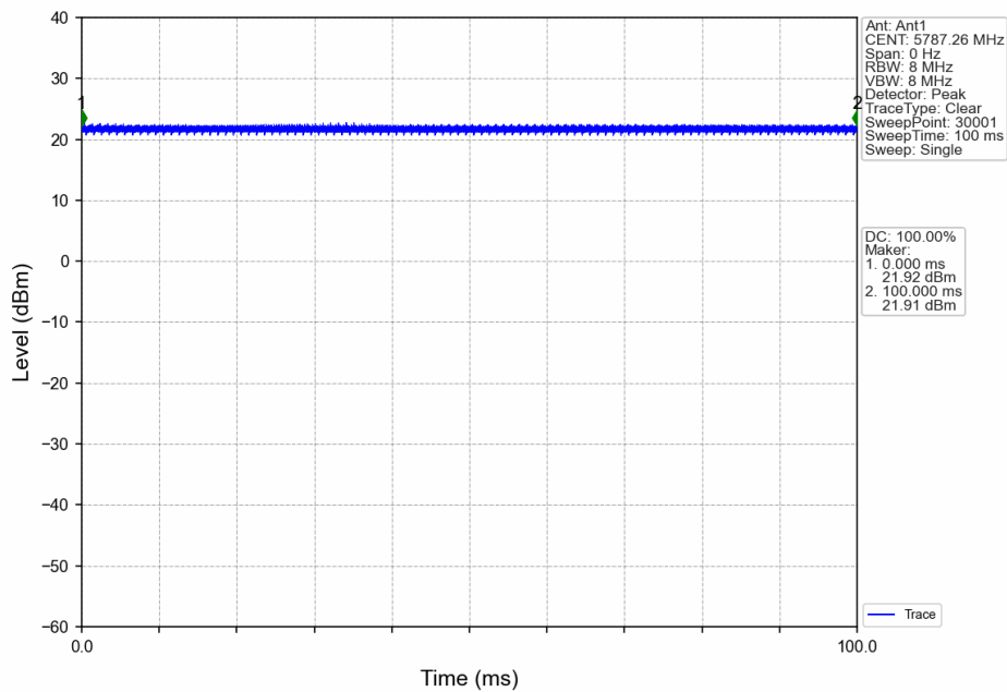
5M_MCH_5787.26MHz_Ant1_NTNV
