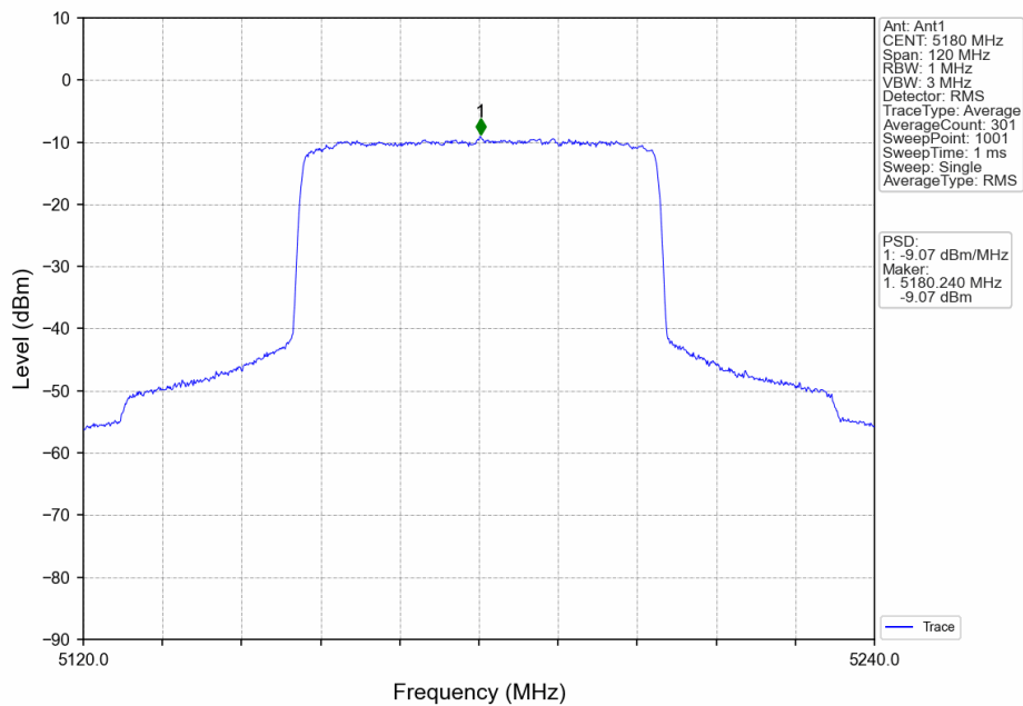
60M_LCH_5180MHz_Ant1_NTNV
