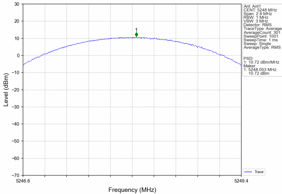
1.4M_HCH_5248MHz_Ant1_NTNV
