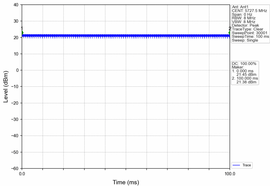
3M_LCH_5727.5MHz_Ant1_NTNV
