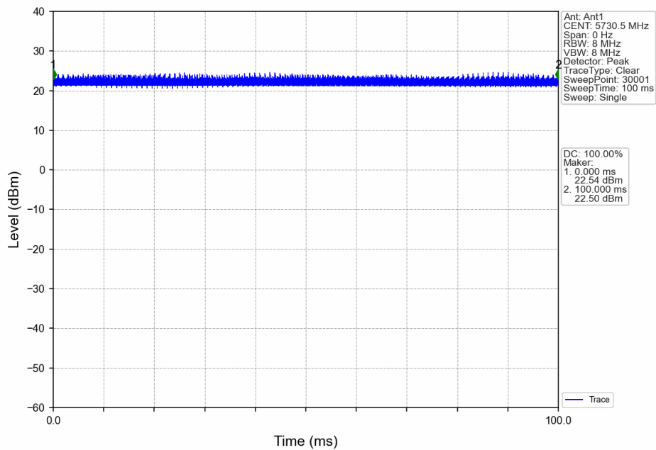
10M_LCH_5730.5MHz_Ant1_NTNV
