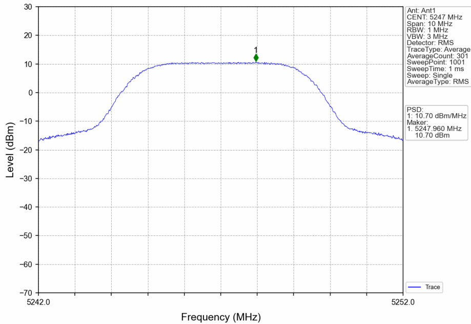
5M_HCH_5247MHz_Ant1_NTNV
