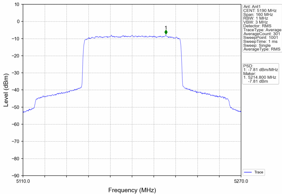
80M_LCH_5190MHz_Ant1_NTNV
