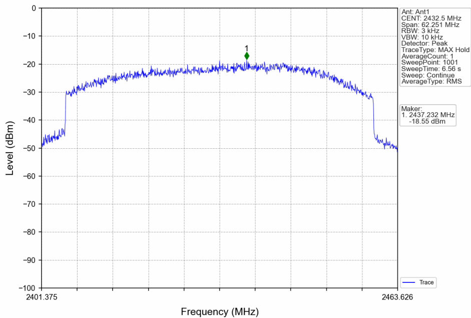
60M_LCH_2432.5MHz_Ant1_NTNV
