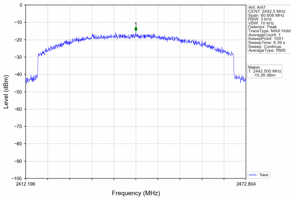
60M_HCH_2442.5MHz_Ant1_NTNV
