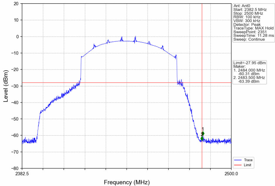
60M_HCH_2442.5MHz_Ant0_NTNV
