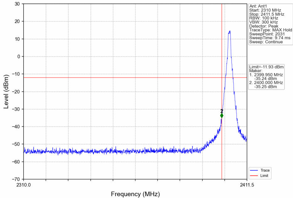
1.4M_LCH_2403.5MHz_Ant1_NTNV
