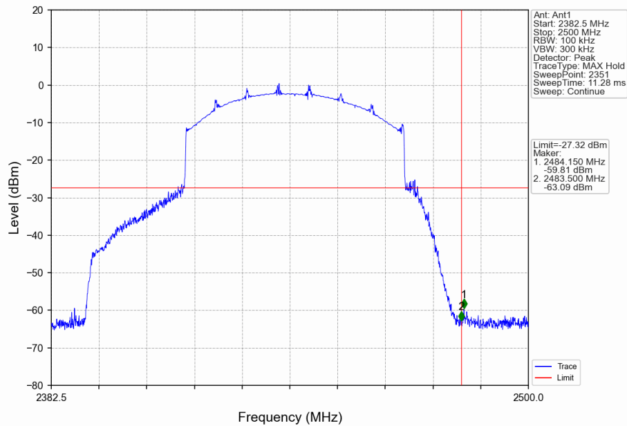
60M_HCH_2442.5MHz_Ant1_NTNV
