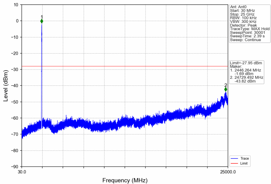
60M_HCH_2442.5MHz_Ant0_NTNV
