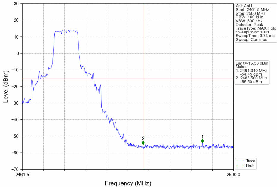
5M_HCH_2469.5MHz_Ant1_NTNV
