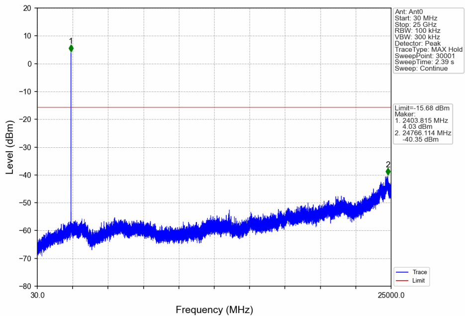
5M_LCH_2404.5MHz_Ant0_NTNV
