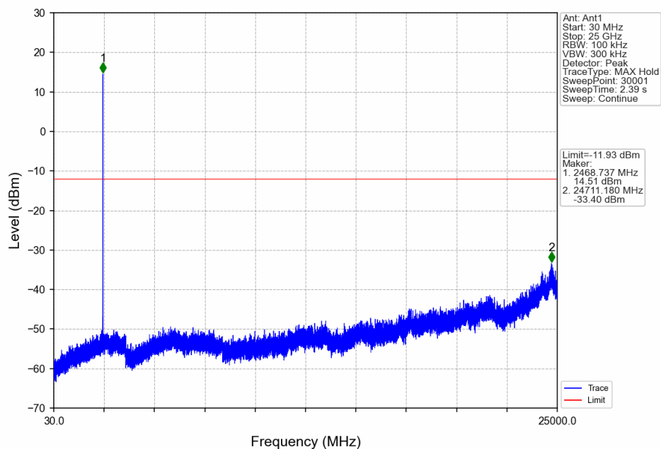
1.4M_HCH_2469.12MHz_Ant1_NTNV
