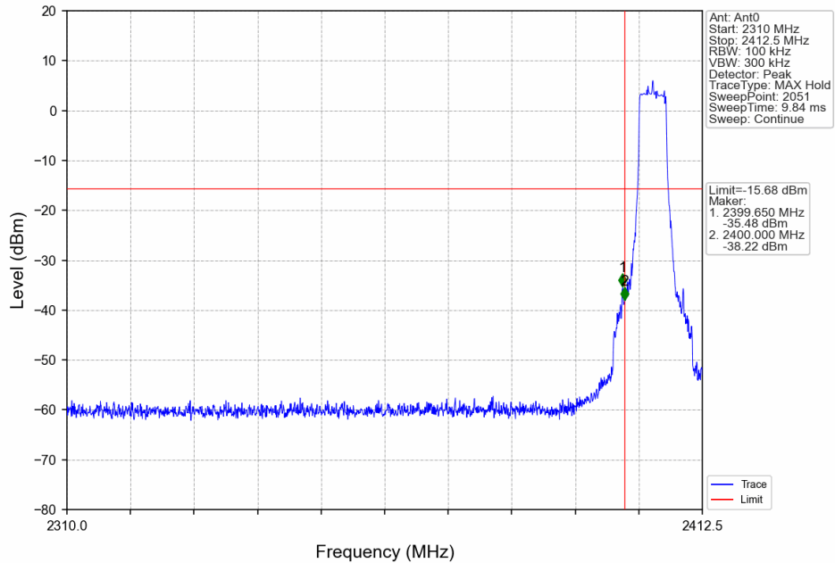
5M_LCH_2404.5MHz_Ant0_NTNV
