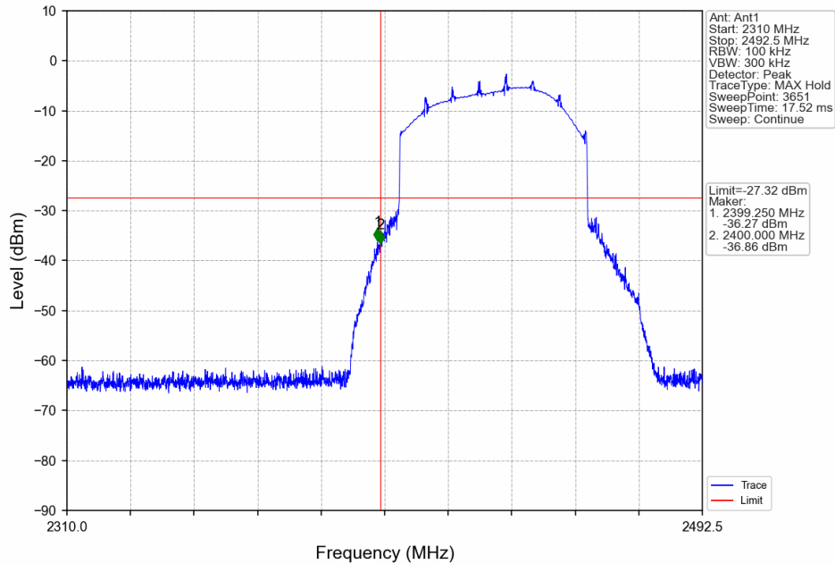
60M_LCH_2432.5MHz_Ant1_NTNV
