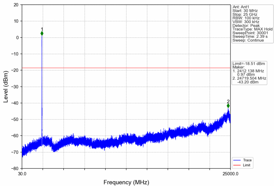
20M_LCH_2412.5MHz_Ant1_NTNV
