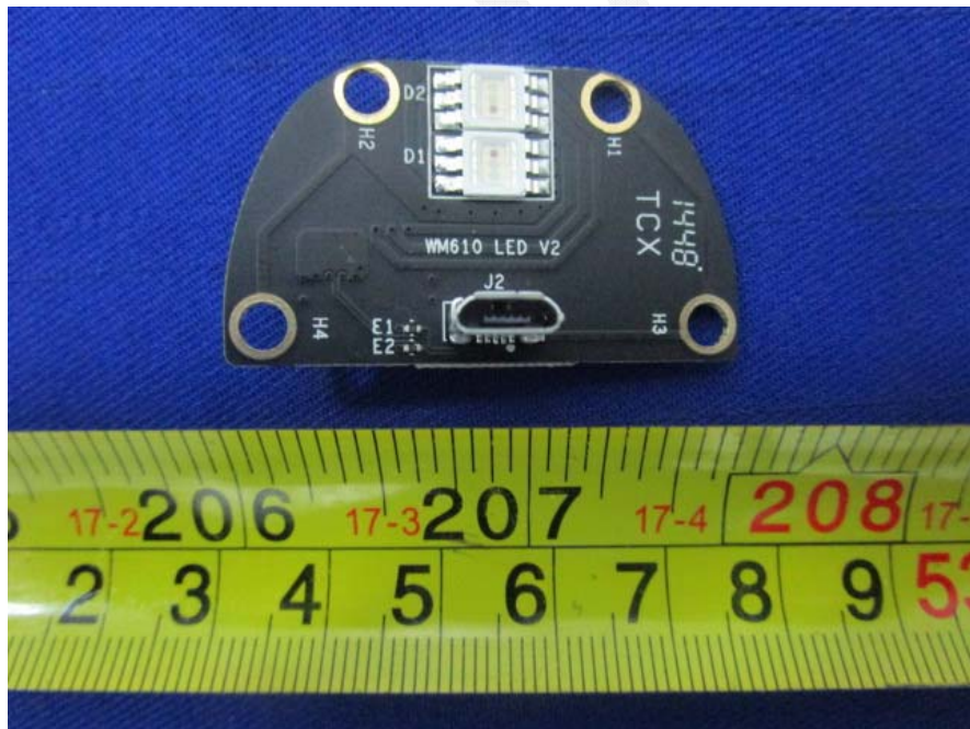
EUT –Light Board Top View
