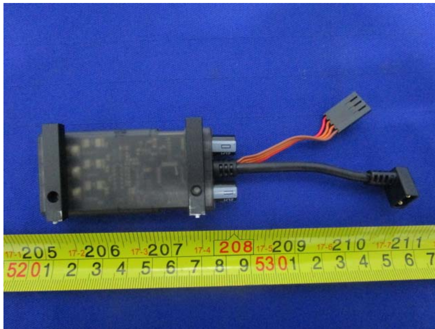
EUT –Turbo Bottom View
