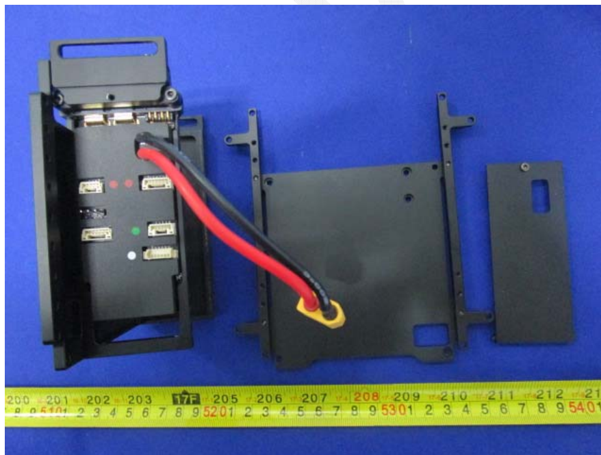
EUT – Power Box Uncover View
