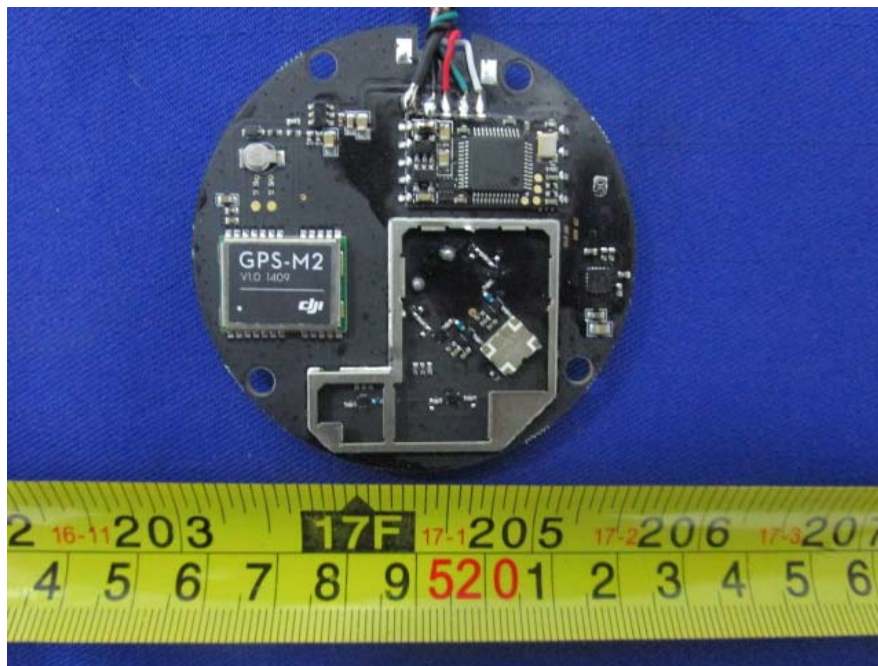
EUT – GPS Top Uncover View
