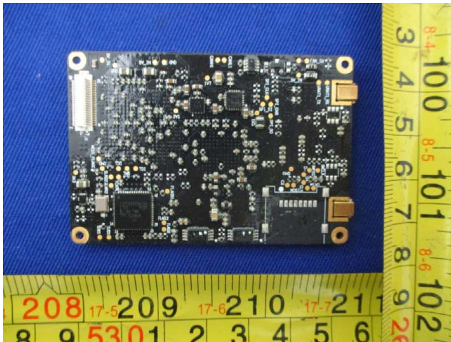
EUT – RF Moudle RF Board Bottom View
