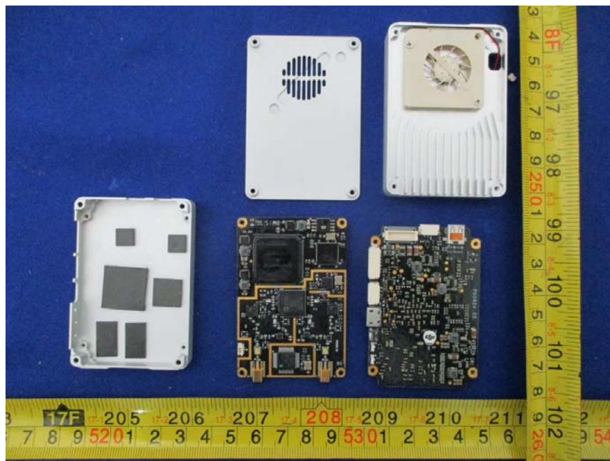
EUT – RF Module Uncover View
