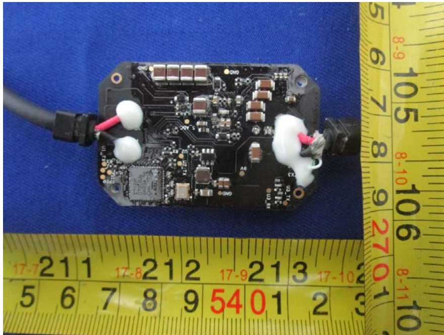
EUT – PMU PRO Module Board Bottom View
