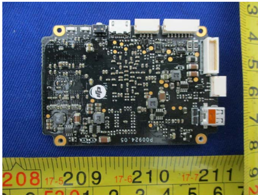
EUT – RF Module Driver Board Bottom View
