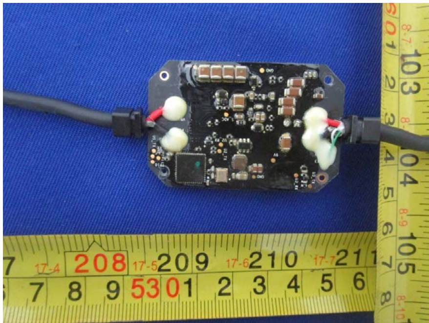
EUT – PMU PRO Module Board Top View
