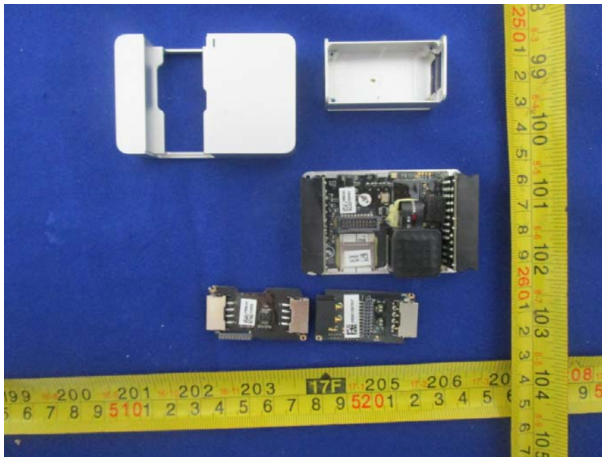
EUT – Flight Controller Module Uncover View
