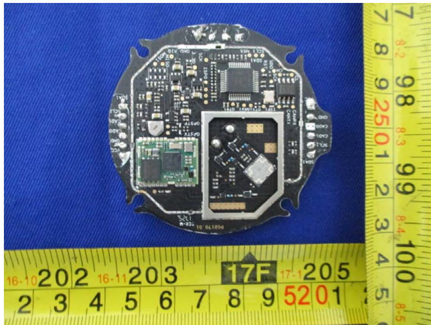
EUT – GPS Module Bottom Unshielded 2 View
