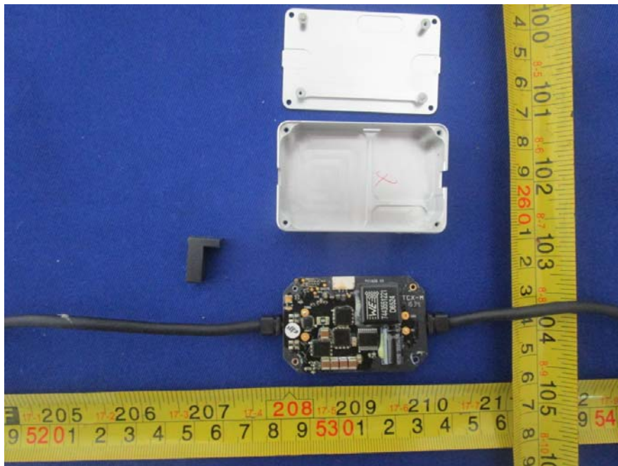
EUT – PMU PRO Module Uncover View
