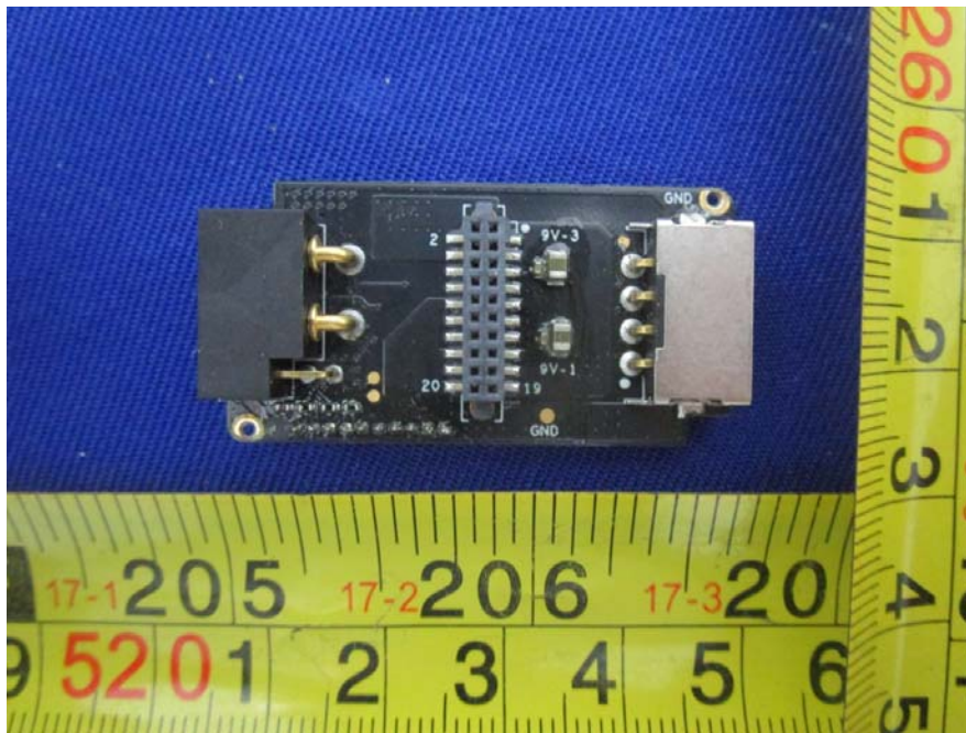
EUT – Flight Controller Module Sub-board-2 Top View
