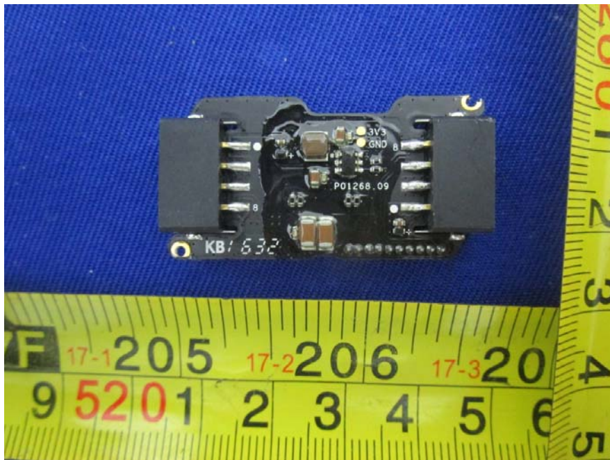
EUT – Flight Controller Module Sub-board-1 Bottom View
