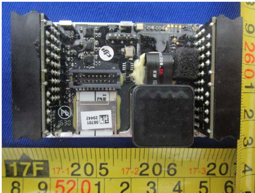
EUT – Flight Controller Module Main Board View
