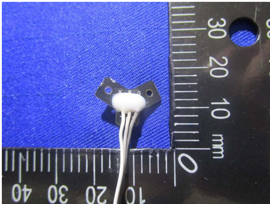
EUT – PCB 14 Bottom View
