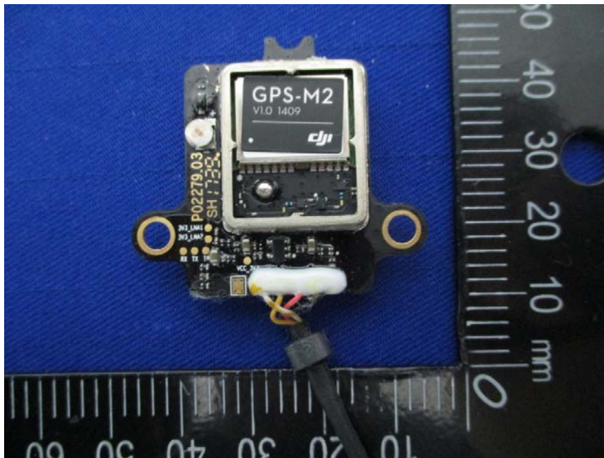
EUT – PCB 9 Bottom Uncover View
