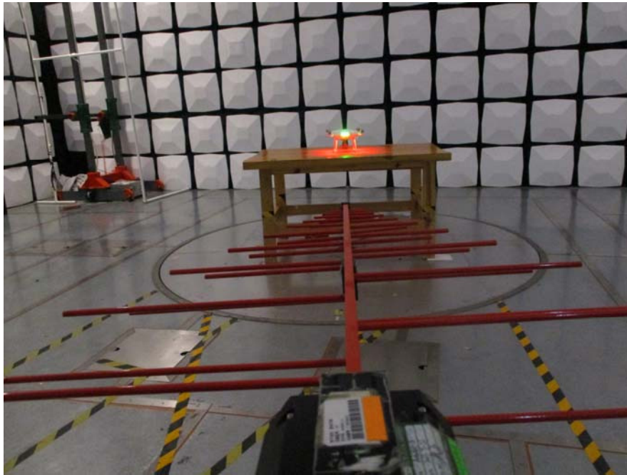
Radiated Emission Operation View (Below 1GHz)
