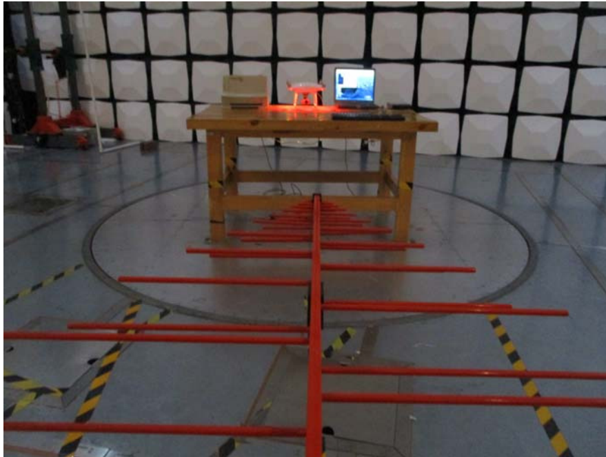
Radiated Emission Downloading Front View (Below 1GHz)
