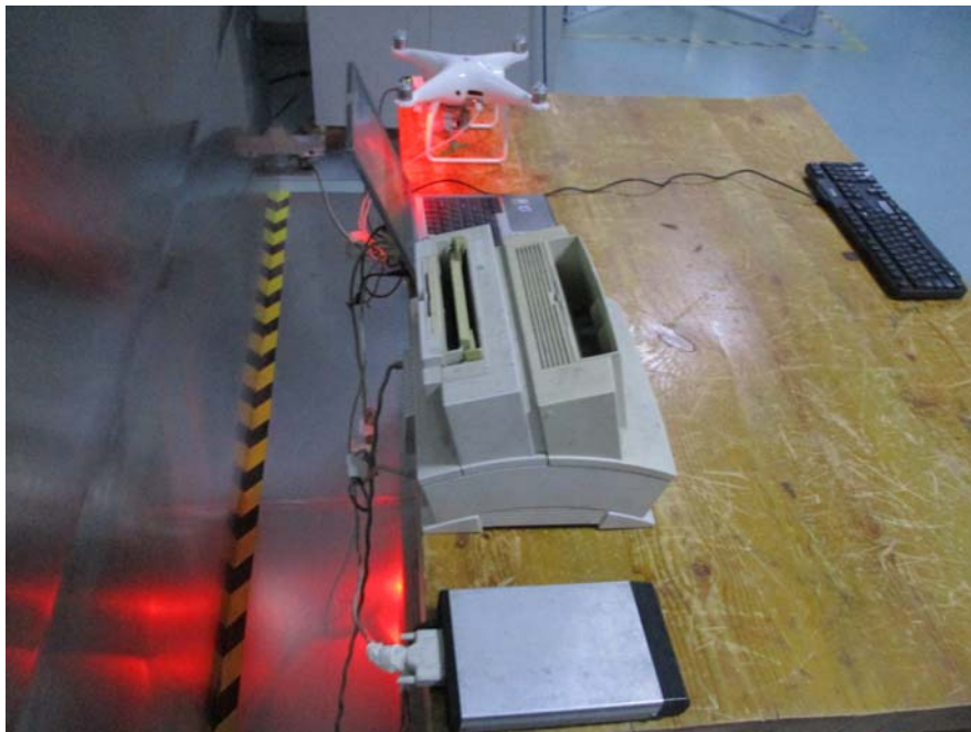
Conducted Emissions – Side View(Downloading)
