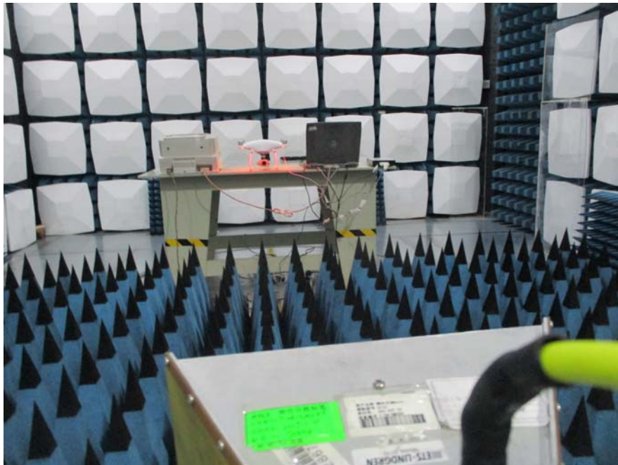
Radiated Emission Downloading Rear View (Above 1GHz)
