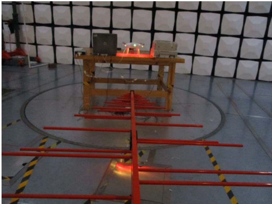
Radiated Emission Downloading Rear View (Below 1GHz)
