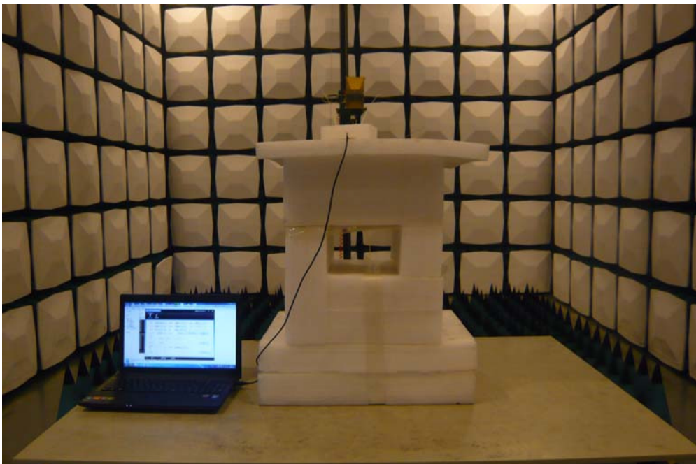
Radiated Emission View—USB Mode (Above 1GHz)
