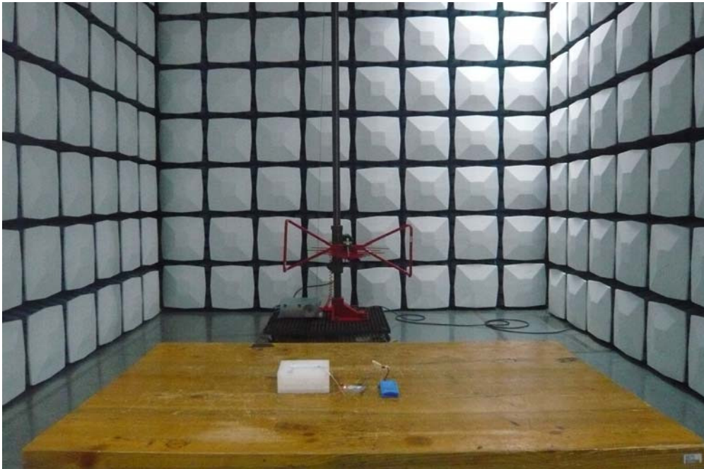
Radiated Emission Battery Mode View (Below 1GHz)
