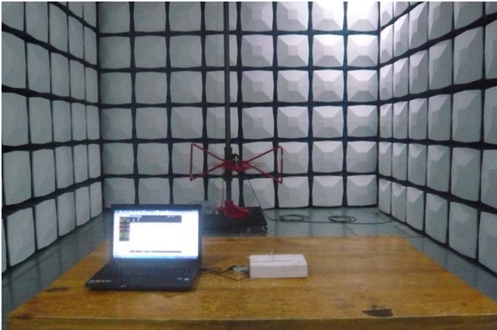
Radiated Emission View—USB Mode (Below 1GHz)
