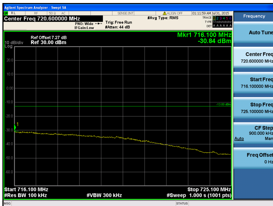
LTE Band 17 / 10MHz / QPSK - RB Size/Offset (50/0)
