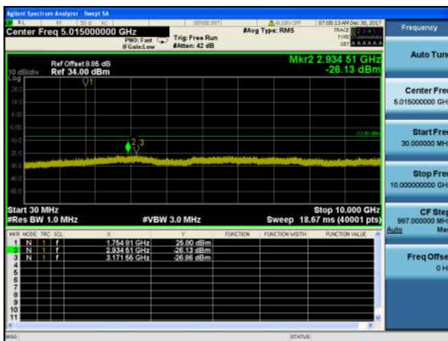
LTE Band 4 / 1.4MHz / 16QAM - RB Size/Offset (3/1) – High Channel
