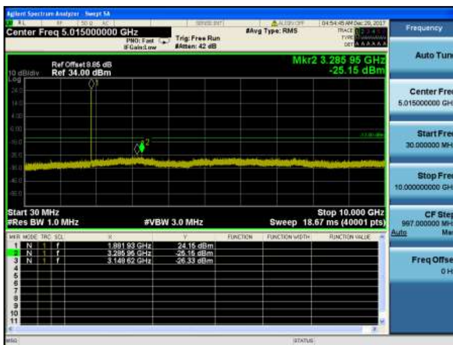
LTE Band 2 / 5MHz / 16QAM - RB Size/Offset (12/13) – Mid Channel
