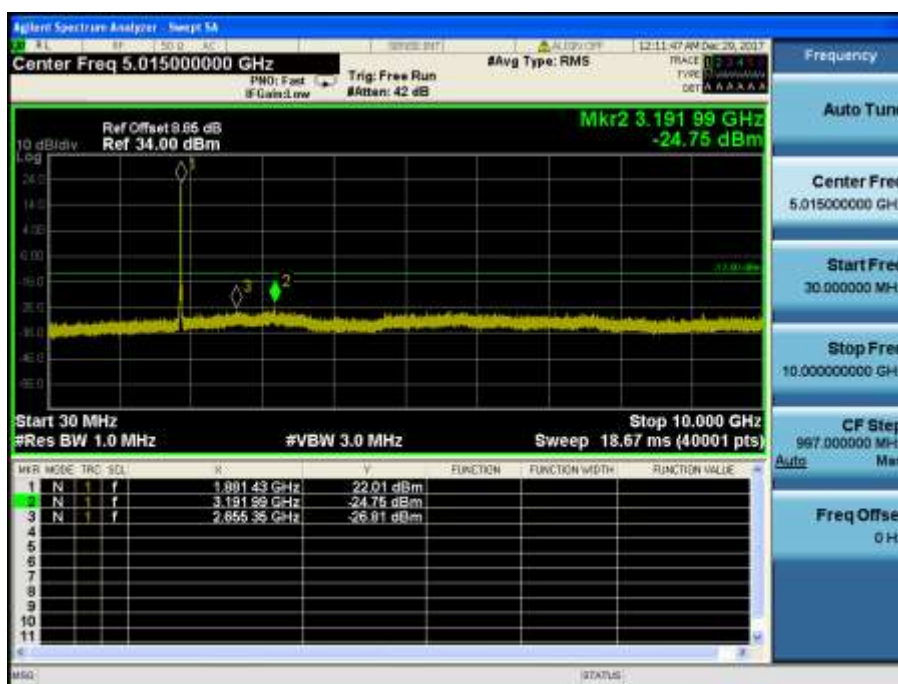
LTE Band 2 / 15MHz / QPSK - RB Size/Offset (36/19) – Mid Channel
