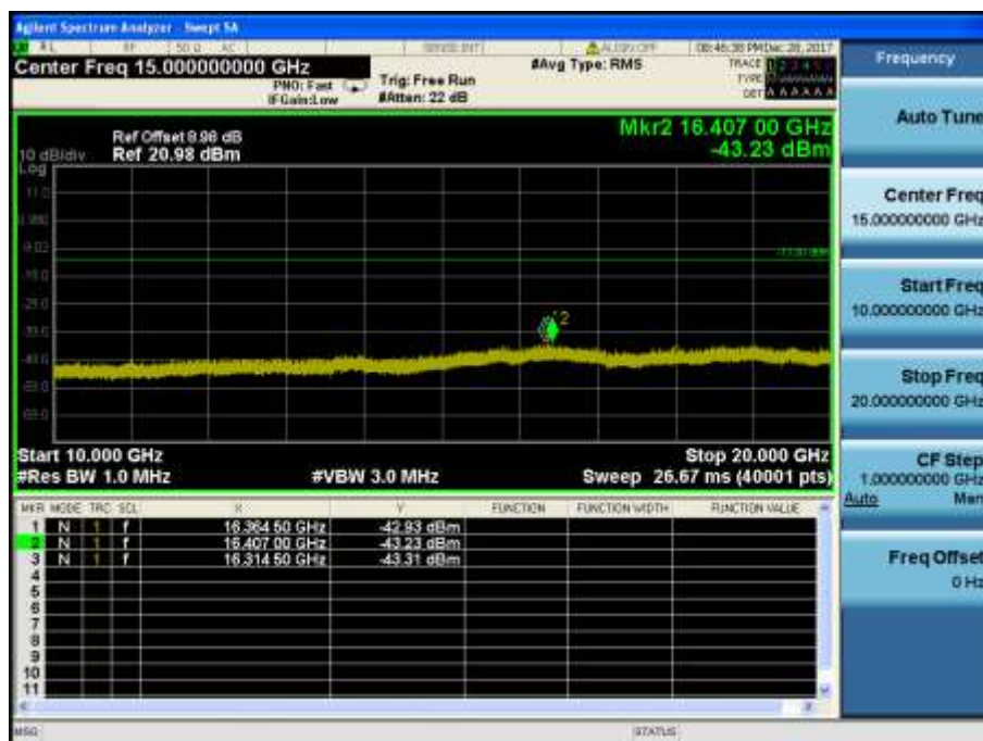
LTE Band 2 / 1.4MHz / QPSK - RB Size/Offset (3/1) – Low Channel
