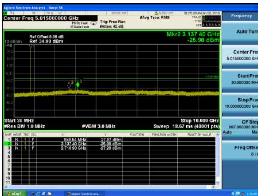
LTE Band 5 / 1.4MHz / 16QAM - RB Size/Offset (1/3) – High Channel
