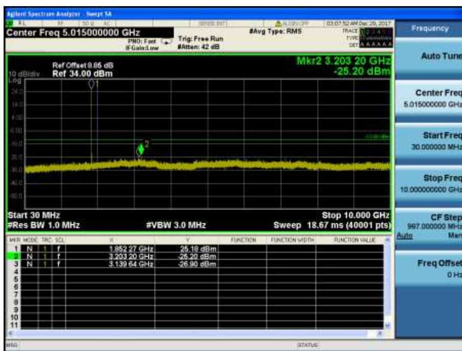
LTE Band 2 / 3MHz / 16QAM - RB Size/Offset (8/7) – Low Channel
