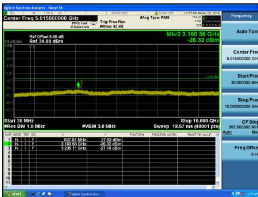
LTE Band 5 / 1.4MHz / 16QAM - RB Size/Offset (3/3) – Mid Channel
