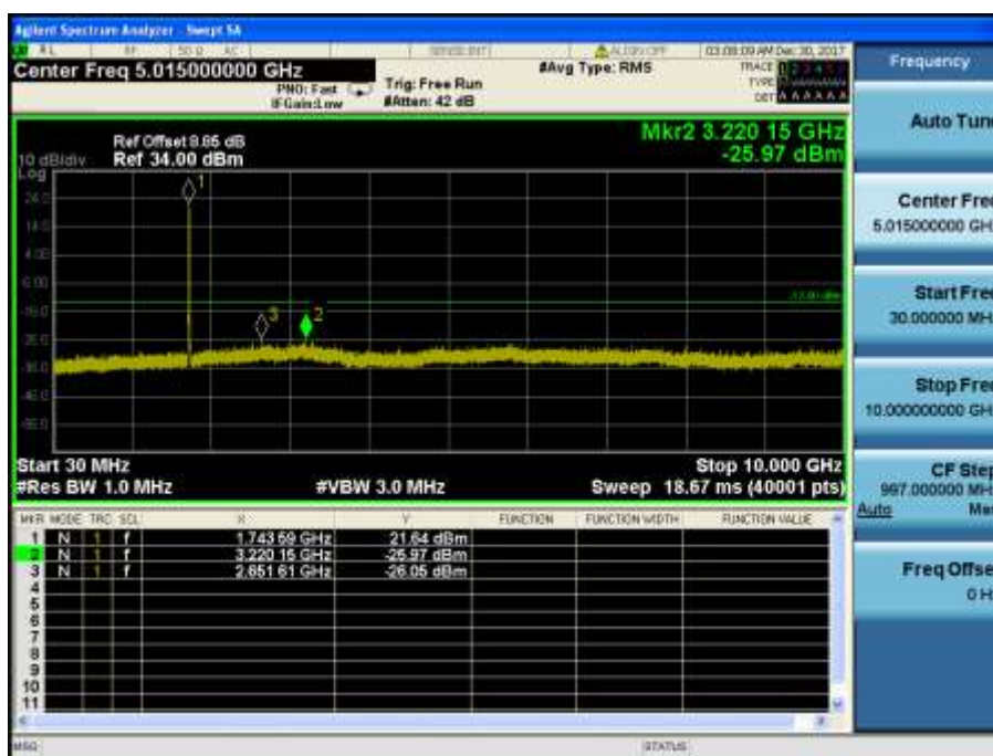
LTE Band 4 / 15MHz / QPSK - RB Size/Offset (36/0) – High Channel
