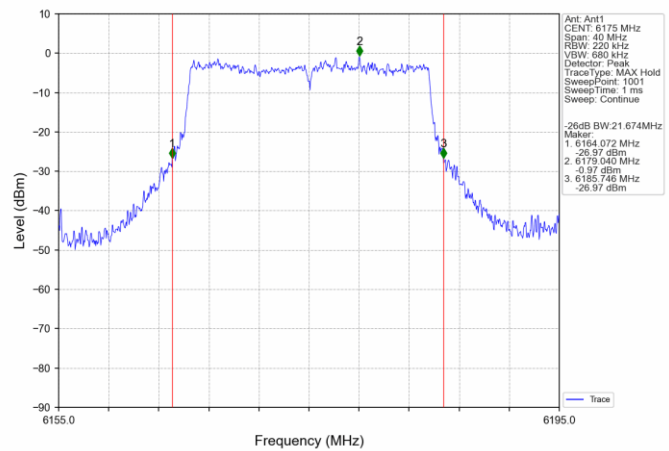
802.11ax(HEW20)_MCH_6175MHz_SU_ / _Ant1_NTNV
