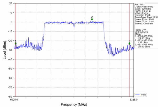
802.11ax(HEW160)_MCH_6185MHz_SU / Ant1_NTNV
