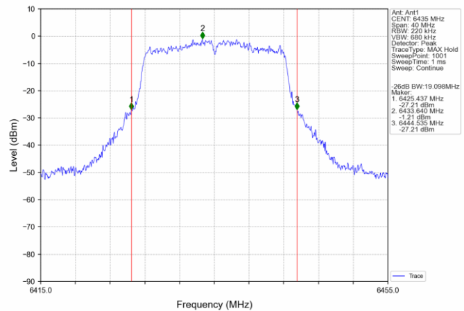
802.11a_LCH_6435MHz_Ant1 NTN
