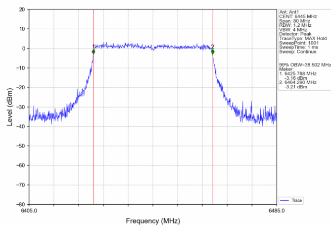
802.11ax(HEW40)_LCH_6445MHz_SU_ / Ant1 NTN
