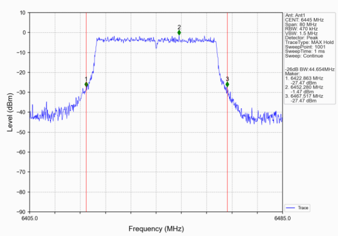
802.11ax(HEW40) LCH_6445MHz_SU / Ant1 NTNv
