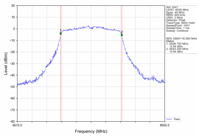
802.11a_LCH_6535MHz_Ant1 NTN
