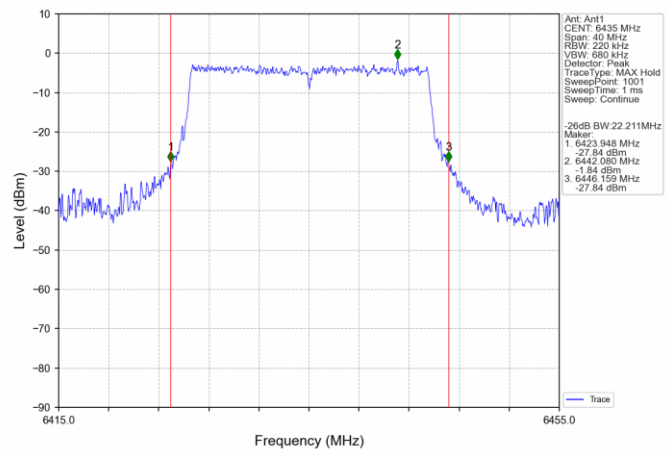
802.11ax(HEW20)_LCH_6435MHz_SU_ / Ant1 NTNv
