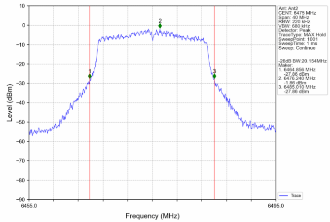
802.11ac(VHT20) MCH 6475MHz Ant2_NTNV
