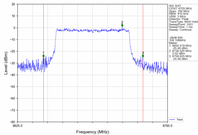
802.11ax(HEW80)_MCH_6705MHz_SU_ / Ant1_NTNV
