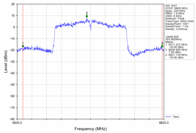
802.11ac(VHT160) MCH 6665MHz Ant1_NTNV
