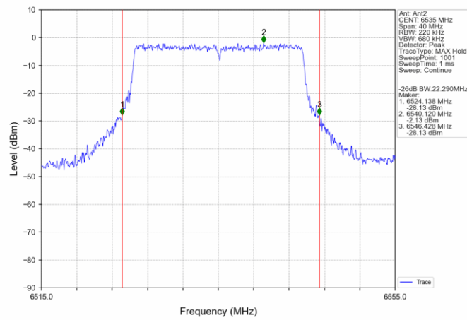
802.11ax(HEW20)_LCH_6535MHz_SU_/_Ant2_NTNV
