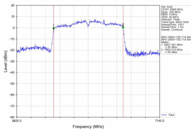
802.11ac(VHT160) MCH_6985MHz_Ant2_NTN
