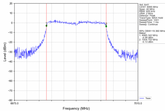
802.11ax(HEW20)_MCH_6995MHz_SU_ / Ant1_NTNV
