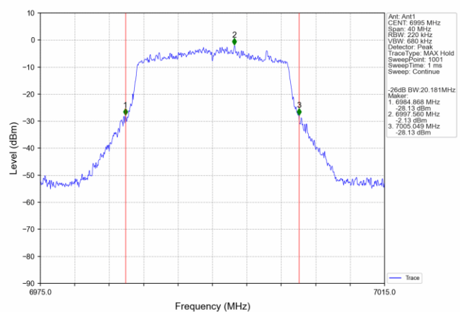
802.11ac(VHT20)_MCH_6995MHz_Ant1_NTNV
