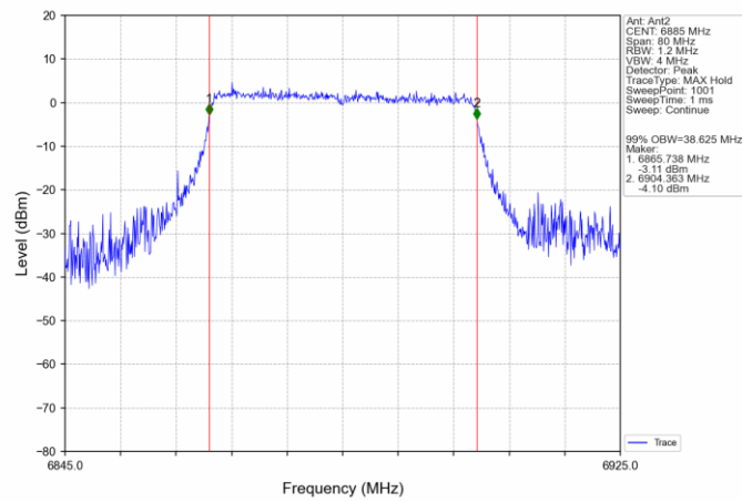
802.11ax(HEW40)_HCH_6885MHz_SU / Ant2_NTNV
