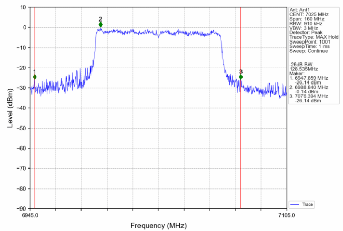
802.11ax(HEW80) HCH_7025MHz_SU_ / Ant1 NTNv
