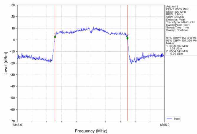
802.11ac(VHT160) HCH_6505MHz_Ant1_NTNV
