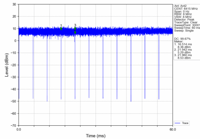
802.11ac(VHT20) HCH_6415MHz_Ant2_NTNV
