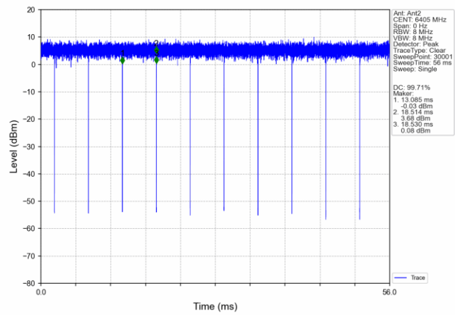
802.11ac(VHT40) HCH_6405MHz_Ant2_NTNV
