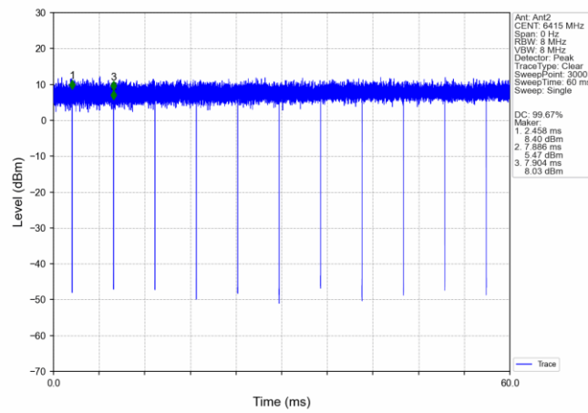
802.11n(HT20) HCH 6415MHz Ant2_NTNV
