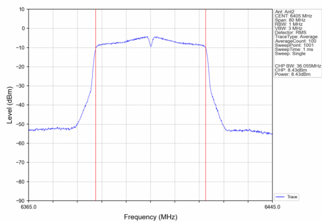
802.11ac(VHT40) HCH_6405MHz_Ant2_NTNV
