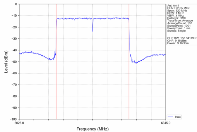
802.11ax(HEW160)_MCH_6185MHz_SU / Ant1_NTNV
