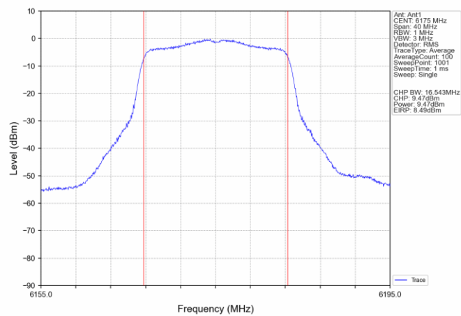
802.11a_MCH_6175MHz_Ant1_NTNV
