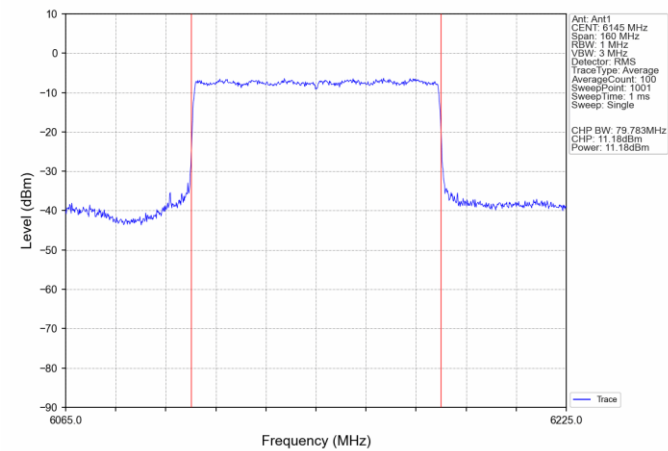
802.11ax(HEW80)_MCH_6145MHz_SU_ / Ant1_NTNV
