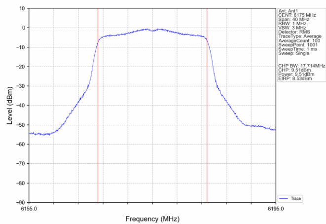
802.11n(HT20)_MCH_6175MHz_Ant1_NTNV
