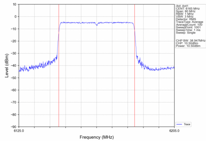
802.11ax(HEW40)_MCH_6165MHz_SU_ / Ant1_NTNV
