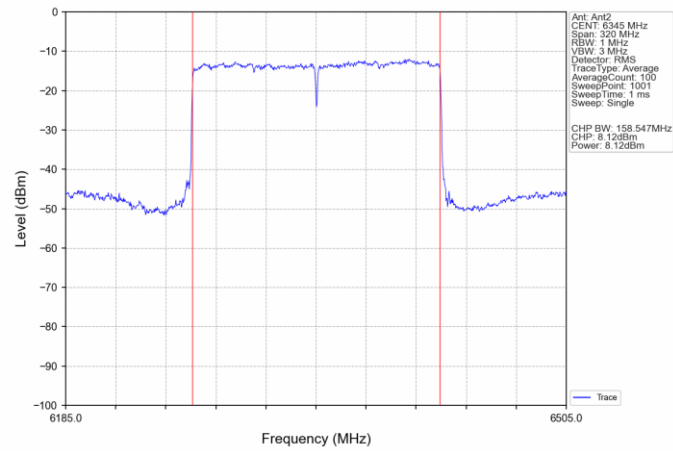
802.11ax(HEW160) HCH 6345MHz_SU / Ant2_NTNV
