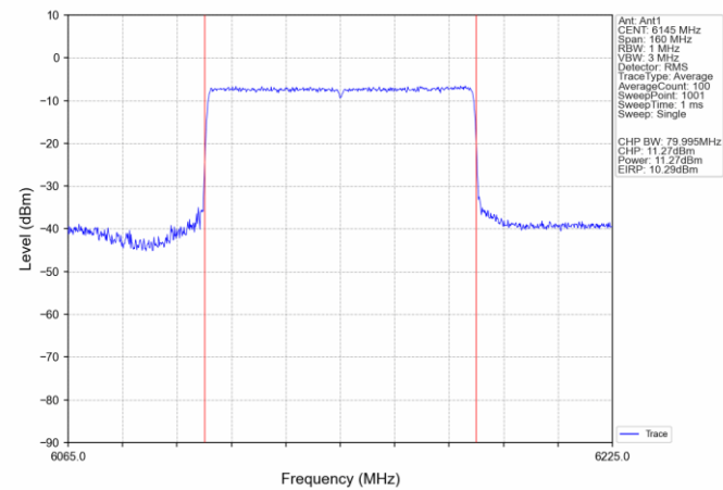
802.11ax(HEW80)_MCH_6145MHz_SU_ / Ant1_NTNV
