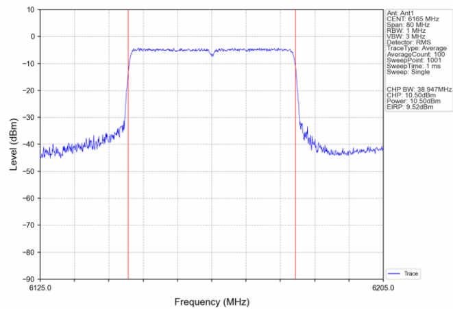
802.11ax(HEW40)_MCH_6165MHz_SU_ / Ant1_NTNV
