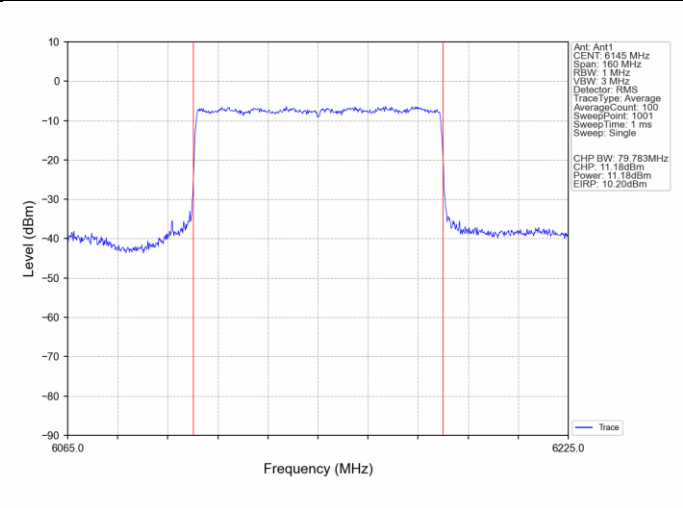
802.11ax(HEW80)_MCH_6145MHz_SU_ / Ant1_NTNV
