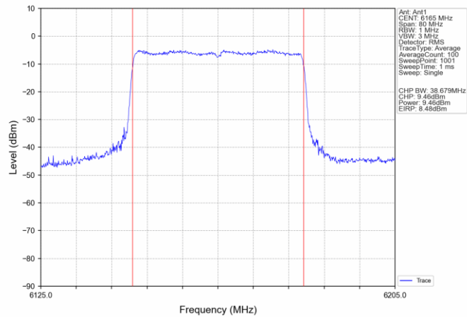
802.11ax(HEW40)_MCH_6165MHz_SU_ / Ant1_NTNV
