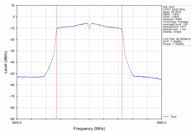
802.11ac(VHT40) LCH_6445MHz_Ant1_NTNV
