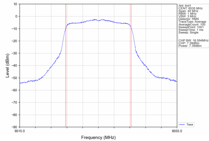
802.11a_LCH_6535MHz_Ant1_NTNV
