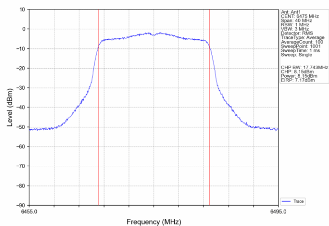
802.11n(HT20) MCH_6475MHz_Ant1_NTNV
