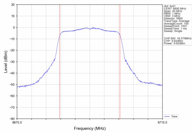
802.11a_MCH_6695MHz Ant1_NTNV
