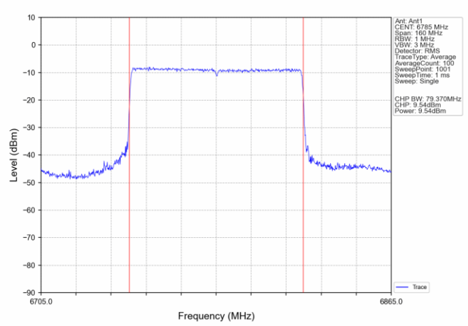
802.11ax(HEW80) HCH_6785MHz_SU_ / Ant1 NTN
